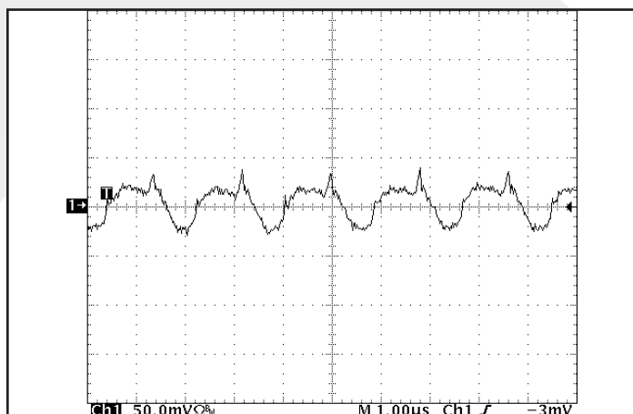
Figure 9: Input terminal current ripple, i_C , at full rated output current and nominal input voltage with SynQor MCOTS filter module (50mA/div). Bandwidth: 20MHz. See Figure 17.
