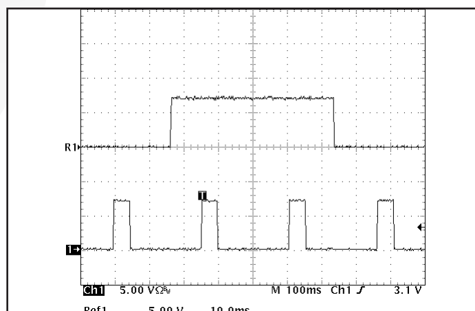
Figure 18: Load current (5A/div) as a function of time (10ms/div and 100ms/div) when the converter attempts to turn on into a 10mΩ short circuit.
