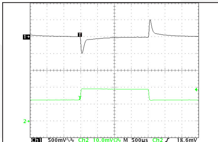
Figure 11: Output voltage response to step-change in load current (50%-75%-50% of I_{out(max)} ; dI/dt = 0.1A/\mu s ). Load cap: 1μF ceramic and 15μF tantalum capacitors. Ch 1: V_{out} (500mV/div), Ch 2: I_{out} (2A/div).
