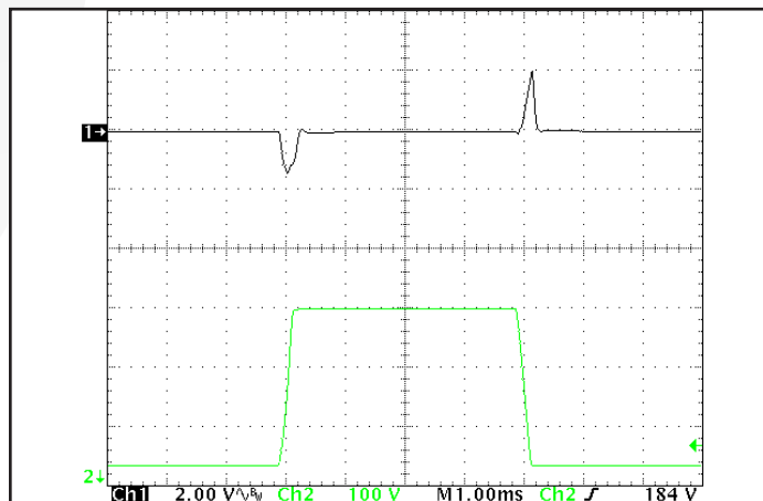
Figure 12: Output voltage response to step-change in input voltage (155V - 425V - 155V) with 250μs rise/fall time. Load cap: 15μF, 100mΩ ESR tantalum cap and 1μF ceramic cap. Ch 1: V_{out} (2000mV/div), Ch 2: V_{in} (100V/div).
