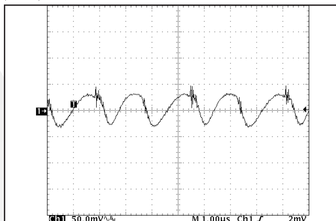
Figure 10: Output voltage ripple, V_{out} , at nominal input voltage and rated load current (50mV/div). Load capacitance: 1μF ceramic capacitor and 10μF tantalum capacitor. Bandwidth: 20MHz. See Figure 17.
