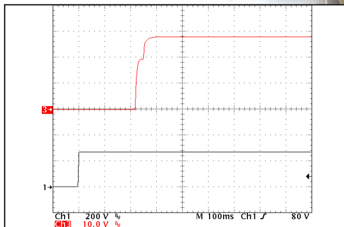
Figure 8: Turn-on transient at full resistive load and zero output capacitance initiated by Vin. ON/OFF Pin previously low. Ch 1: Vin (200V/div). Ch 3: Vout (10V/div).
