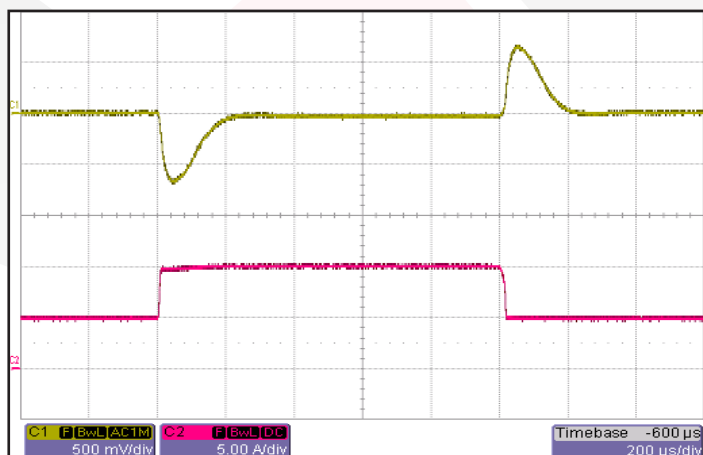
Figure 11: Output voltage response to step-change in load current 50%-100%-50% of I_{out} (max). Load cap: 1 \mu F ceramic cap and 10 \mu F, 100m \Omega ESR tantalum cap. Ch 1: V_{out} (500mV/div). Ch 2: I_{out} (5A/div).
