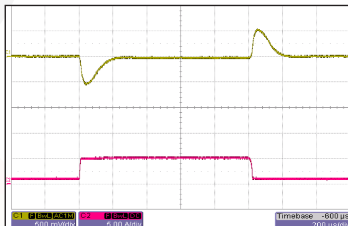
Figure 12: Output voltage response to step-change in load current 10%-50%-10% of I_{out} (max). Load cap: 1 \mu F ceramic cap and 10 \mu F, 100m \Omega ESR tantalum cap. Ch 1: V_{out} (500mV/div). Ch 2: I_{out} (5A/div).
