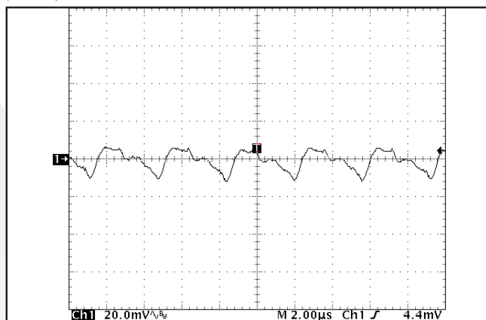
Figure 10: Output voltage ripple, Vout, at nominal input voltage and rated load current (20mV/div). Load capacitance: 1μF ceramic capacitor and 10μF tantalum capacitor. Bandwidth: 20 MHz. See Figure 17.
