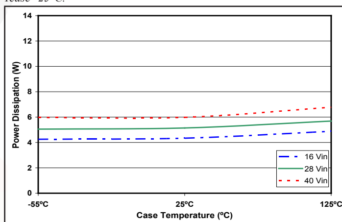
Figure 6: Power Dissipation at 60% load (0.99A load on +15V and 0.99A load on -15V) versus case temperature for V_{in} = 16V, 28V and 40V .
