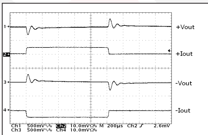
Figure 17: Output voltage response to step-change in total load current (0%-50%-0%) of total Iout (max) split 50%/50%. Load cap: 1 \mu F ceramic cap and 10 \mu F, 100m \Omega ESR tantalum cap. Ch 1: +Vout (500mV/div); Ch 2: +Iout (2A/div); Ch 3: -Vout (500mV/div); Ch 4: -Iout (2A/div).
