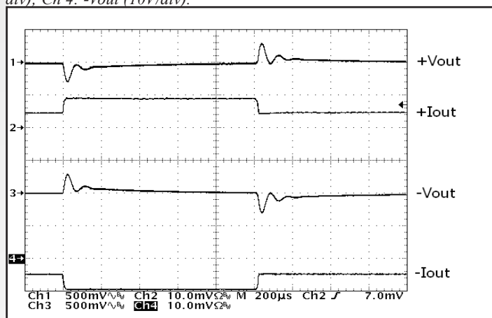
Figure 16: Output voltage response to step-change in total load current (50%-100%-50%) of total Iout (max) split 50%/50%. Load cap: 1 \mu F ceramic cap and 10 \mu F, 100m \Omega ESR tantalum cap. Ch 1: +Vout (500mV/div); Ch 2: +Iout (2A/div); Ch 3: -Vout (500mV/div); Ch 4: -Iout (2A/div).
