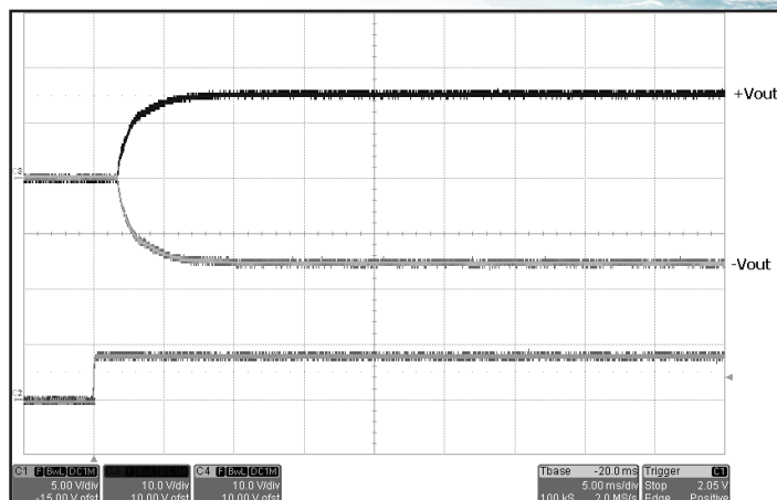
Figure 14: Turn-on transient at zero load current (5ms/div). Input voltage pre-applied. Ch 1: Enable input (5V/div); Ch 3: +Vout (10V/div); Ch 4: -Vout (10V/div).
