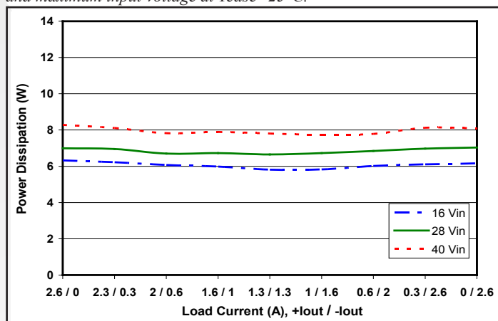
Figure 4: Power dissipation vs. output power, with total output current fixed at 80% load (40W) and loads split as shown between the +15V and -15V outputs at minimum, nominal, and maximum input voltage at T_{case}=25^{\circ}C .
