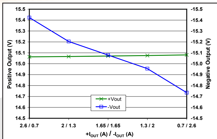
Figure 7: Load regulation vs. load current with power fixed at full load (50W) and load currents split as shown between the +15V and -15V outputs, at nominal input voltage and T_{case} = 25^{\circ}C .
