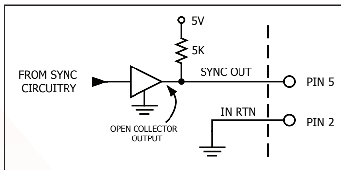
Figure C: Equivalent circuit looking into the SYNC OUT pin with respect to the IN RTN (input return) pin.
