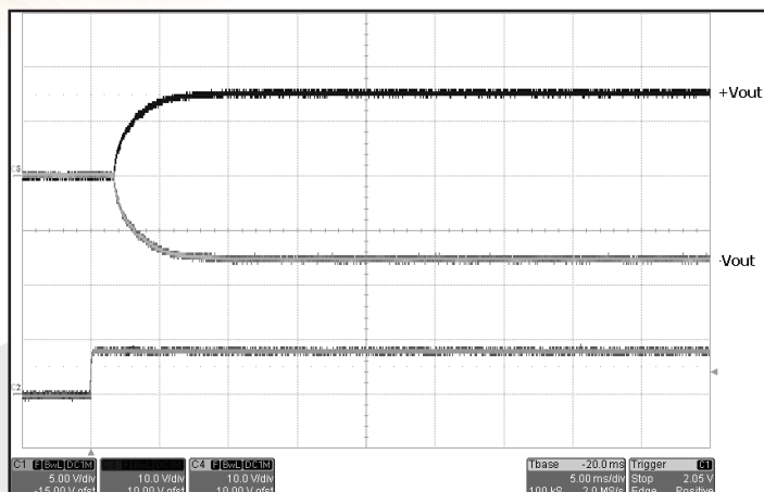
Figure 13: Turn-on transient at full load current (resistive load) (5 ms/div). Input voltage pre-applied. Ch 1: Enable input (5V/div); Ch 3: +Vout (10V/div); Ch 4: -Vout (10V/div).
