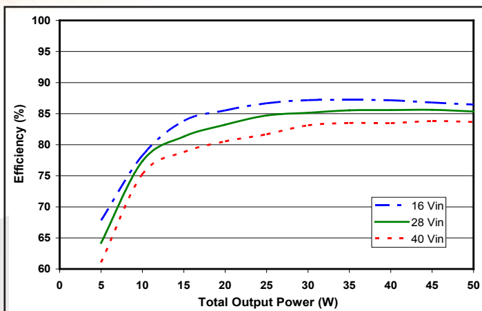
Figure 1: Efficiency vs. output power, from zero load to full load with equal load on the +15V and -15V outputs at minimum, nominal, and maximum input voltage at T_{case}=25^{\circ}C .
