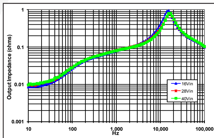
Figure 24: Magnitude of incremental output impedance of +15V output ( +Z_{out} = +v_{out}/+i_{out} ) for minimum, nominal, and maximum input voltage at full rated power.
