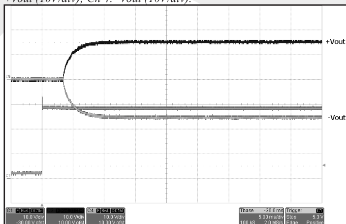
Figure 15: Turn-on transient at full load current, after application of input voltage (ENA logic high) (5ms/div). Ch 1: Vin (10V/div); Ch 3: +Vout (10V/div); Ch 4: -Vout (10V/div).
