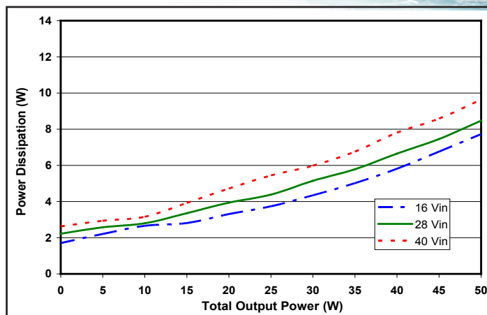
Figure 2: Power dissipation vs. output power, from zero load to full load with equal load on the +15V and -15V outputs at minimum, nominal, and maximum input voltage at T_{case}=25^{\circ}C .
