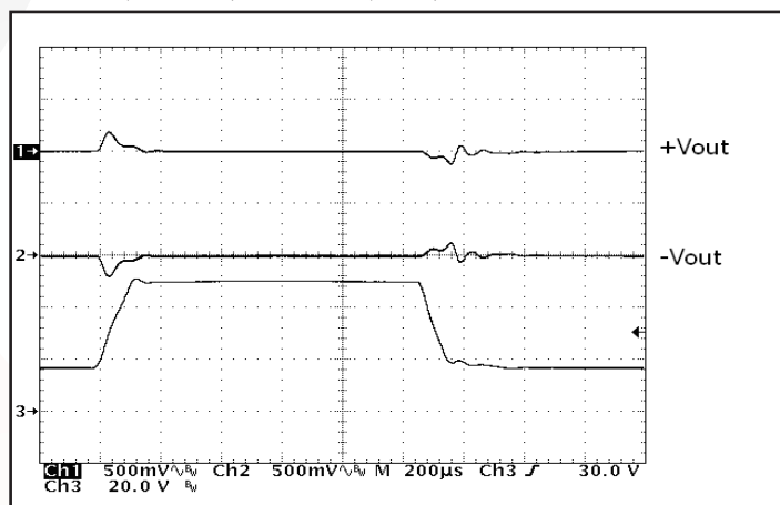
Figure 18: Output voltage response to step-change in input voltage (16V-50V-16V). Load cap: 1 \mu F ceramic cap and 10 \mu F, 100m \Omega ESR tantalum cap. Ch 1: +Vout (500mV/div); Ch 2: -Vout (500mV/div); Ch 3: Vin (20V/div).
