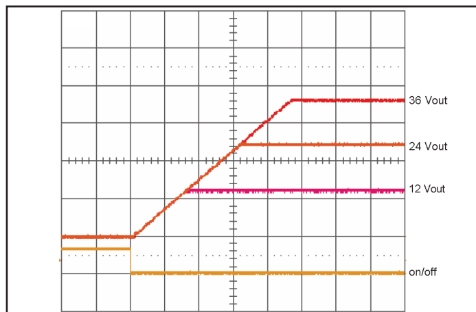
Figure 8: Turn-on transient at 24V input; zero load (20ms/div). ON/OFF input (5V/div) Ch 1-3: Vout (10V/div)
