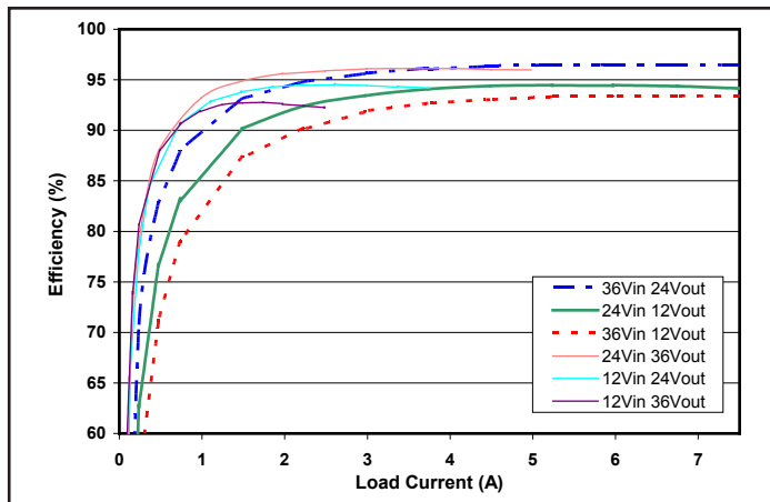
Figure 1: Efficiency at nominal output voltage vs. load current for nominal input voltage at 25 °C.
