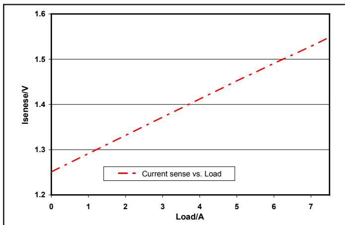
Figure 9: Imon pin voltage vs. load current at 24V input and 13.8V output. Load capacitance: 100μF electrolytic cap. C option only
