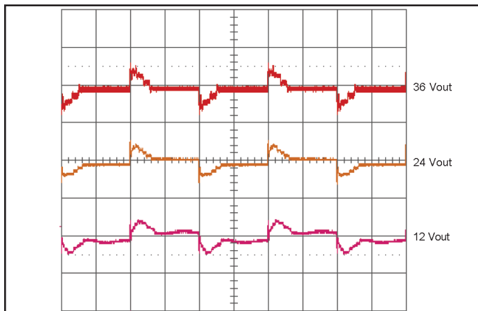
Figure 11: Output voltage response for 24V input; 12V, 24V, 36V output to step-change in load current (50-75-50% of Iout max; di/dt=0.1A/μs). Load cap: 100μF, 100mΩ ESR tant, Ch 1-3: Vout (2V/div);(5ms/div).
