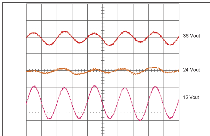
Figure 5: Input Terminal Ripple Current at 24V input and rated load current (500mA/div). Bandwidth: 20MHz. See Figure 4.
