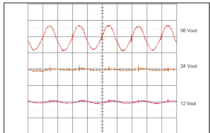
Figure 6: Output Voltage Ripple at 24V input and rated load current (50mV/div). Zero load capacitance. Bandwidth: 20MHz. See Figure 4.
