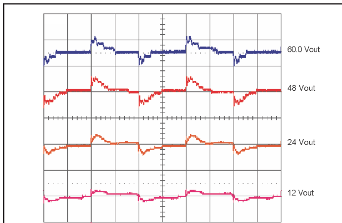
Figure 11: Output voltage response for 24V input; 12V, 24V, 48V, 60V output to step-change in load current (50-75-50% of Iout max; di/dt=0.1A/µs). Load cap: 100µF, 100mΩ ESR tant, Ch 1-4: Vout (1V/div);(5ms/div).
