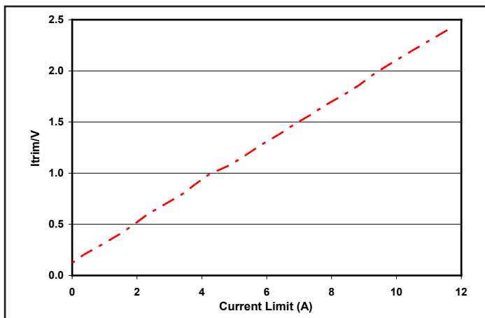
Figure 10: Current limit vs. Itrim pin voltage with 24V input voltage and 13.8V output voltage. Load capacitance: 100µF electrolytic cap.
