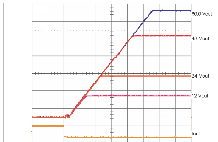
Figure 8: Turn-on transient at full load (resistive load) (50ms/div). ON/OFF input (5V/div) Ch 1-4: Vout (10V/div)
