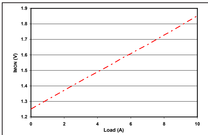
Figure 9: Imon pin voltage vs. load current at 24V input and 13.8V output. Load capacitance: 100µF electrolytic cap. C option only.
