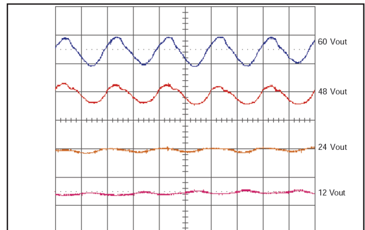
Figure 6: Output Voltage Ripple at 36V input and rated load current (50mV/div). Load capacitance: 100 \mu F electrolytic cap.. Bandwidth: 20MHz. See Figure 4.
