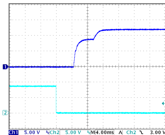
Figure 14: Turn-on transient at zero load (4 ms/div). Ch 1: Vout (5V/div). Ch 2: ON/OFF input (5V/div).
