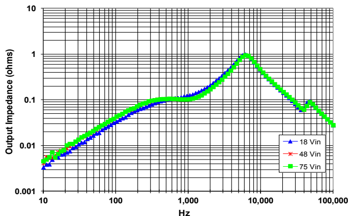
Figure 23: Magnitude of incremental output impedance ( Z_{out} = v_{out}/i_{out} ) for minimum, nominal, and maximum input voltage at full rated power.
