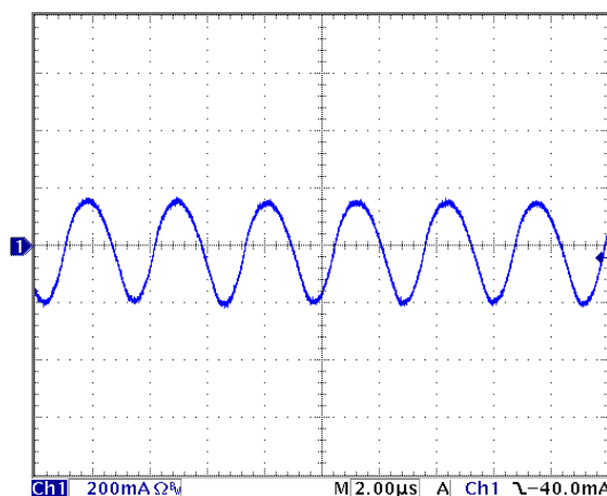
Figure 18: Input Terminal Ripple Current, i c , at full rated output current and nominal input voltage with 10μH source impedance and 47μF electrolytic capacitor (200 mA/div). See Figure 17.
