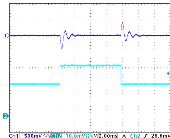
Figure 16: Output voltage response to step-change in load current (50%-75%-50% of Iout(max); dI/dt = 5A/μs). Load cap: 470μF, 30 mW ESR tantalum cap and 1μF ceramic cap. Ch 1: Vout (500mV/div), Ch 2: Iout (2A/div).
