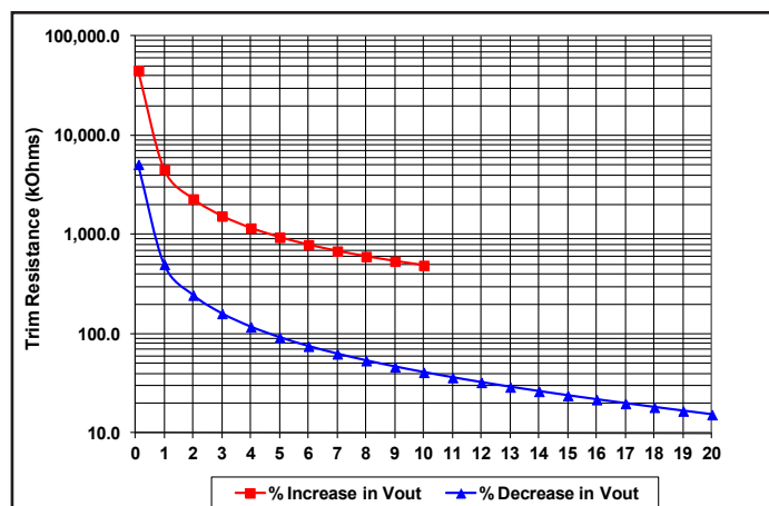
Figure C: Trim Graph
