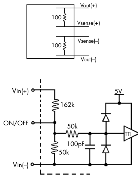
Figure B: Internal ON/OFF pin circuitry
