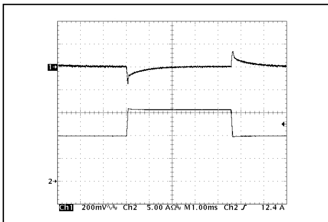
Figure 15: Output voltage response to step-change in load current (50%-75%-50% of I_{out(max)} ; dI/dt = 0.1A/\mu s ). Load cap: 10 \mu F, 100 m \Omega ESR tantalum capacitor and 1 \mu F ceramic capacitor. Ch 1: Vout (200mV/div), Ch 2: Iout (5A/div).
