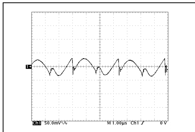
Figure 20: Output voltage ripple at nominal input voltage and rated load current (50 mV/div). Load capacitance: 1 \mu F ceramic capacitor and 10 \mu F tantalum capacitor. Bandwidth: 20 MHz. See Figure 17.
