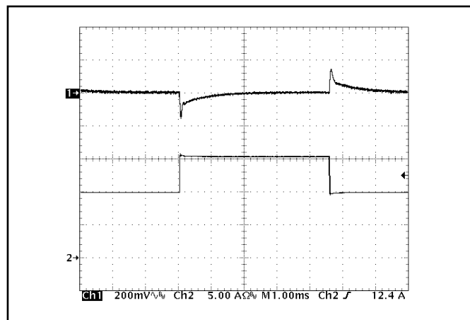
Figure 16: Output voltage response to step-change in load current (50%-75%-50% of I_{out(max)} ; dI/dt = 5A/\mu s ). Load cap: 470 \mu F, 30 m \Omega ESR tantalum capacitor and 1 \mu F ceramic cap. Ch 1: Vout (200mV/div), Ch 2: Iout (5A/div).
