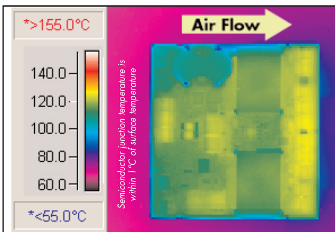
Figure 6: Thermal plot of converter at 96 amp load current with 55°C air flowing at the rate of 200 LFM. Air is flowing across the converter from input to output (nominal input voltage).
