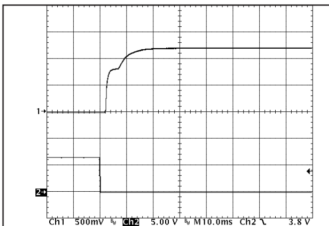
Figure 10: Turn-on transient at zero load (10 ms/div). Top Trace: V_{out} (500mV/div) Bottom Trace: ON/OFF input (5V/div)
