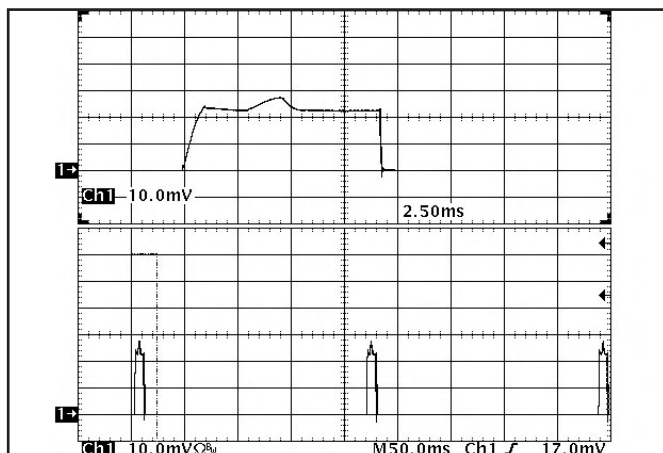
Figure 18: Load current (50A/div) as a function of time when the converter attempts to turn on into a 1\text{m}\Omega short circuit. Top trace (2.5ms/div) is an expansion of the on-time portion of the bottom trace.
