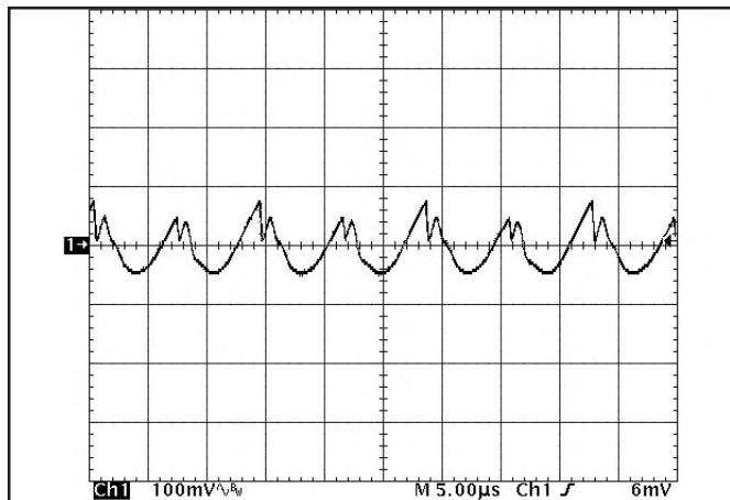
Figure 16: Output voltage ripple at nominal input voltage and rated load current (100 mV/div). Load capacitance: 1\mu\text{F} ceramic capacitor and 15\mu\text{F} tantalum capacitor. Bandwidth: 20 MHz. (See Figure 13)
