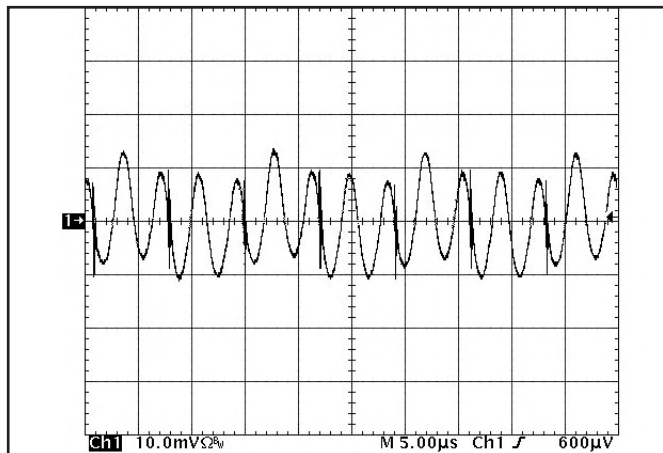
Figure 14: Input Terminal Ripple Current, i_c , at full rated output current and nominal input voltage with 10\mu\text{H} source impedance and 47\mu\text{F} electrolytic capacitor (100 mA/div). (See Figure 13)
