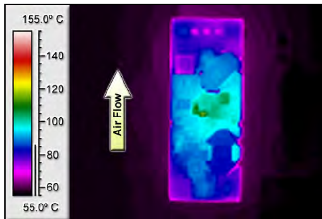
Figure 8: Thermal plot of converter at 6.25 amp load current (75W) with 55°C air flowing at the rate of 200 LFM. Air is flowing across the converter from input to output (nominal input voltage).
