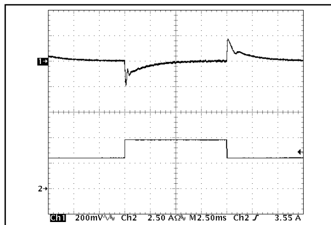
Figure 12: Output voltage response to step-change in load current (50%-75%-50% of I_{out(max)} ; dI/dt = 1A/\mu s ). Load cap: 470 \mu F , 30 m \Omega ESR tantalum cap and 1 \mu F ceramic cap. Ch 1: V_{out} (200mV/div), Ch 2: I_{out} (2.5A/div).
