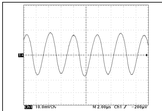
Figure 14: Input Terminal Ripple Current, i_c , at full rated output current and nominal input voltage with 10\ \mu H source impedance and 47\ \mu F electrolytic capacitor (200 mA/div). See Figure 13.
