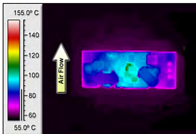
Figure 6: Thermal plot of converter at 6.25 amp load current (75W) with 55°C air flowing at the rate of 200 LFM. Air is flowing across the converter from pin 3 to pin 1 (nominal input voltage).
