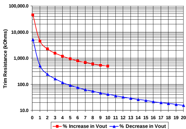
Figure C: Trim Graph for 12Vout module
