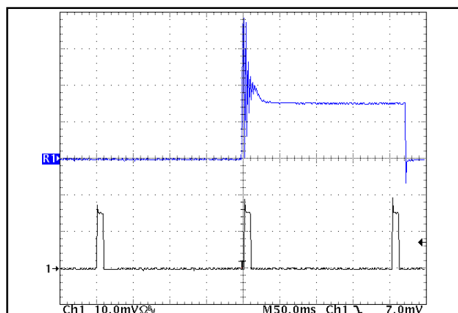
Figure 18: Load current (5A/div) as a function of time when the converter attempts to turn on into a 10\ m\Omega short circuit. Top trace (2.0ms/div) is an expansion of the on-time portion of the bottom trace.
