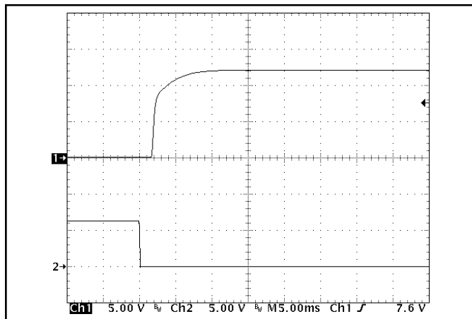
Figure 9: Turn-on transient at full load (resistive load) (5 ms/div). Input voltage pre-applied. Ch 1: V_{out} (5V/div). Ch 2: ON/OFF input (5V/div)
