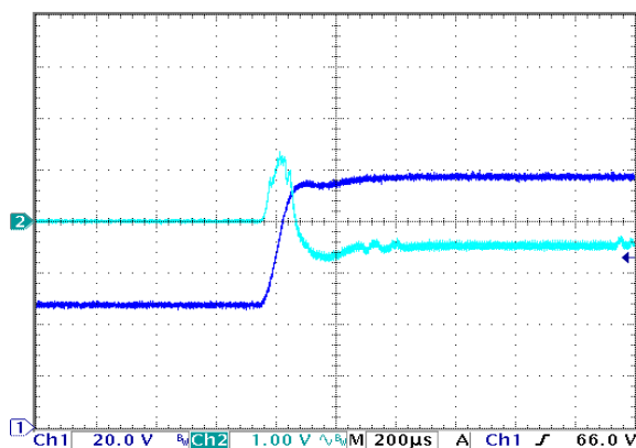
Figure 15: Output voltage response to step-change in input voltage (50V to 100V in 200µs). Load cap: 470µF, 15 mW ESR tantalum capacitor. Ch 1: V_{in} (20V/div), Ch 2: V_{out} (1V/div), at zero load current.
