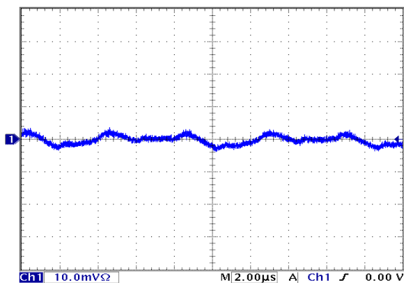
Figure 13: Input reflected ripple current, is, through a 4.7µH source inductor, using a 100µF input capacitor, at nominal input voltage and rated load current (10mA/div). See Figure 11.
