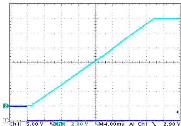
Figure 7: Turn-on transient at full load (resistive load) (4ms/div). Ch 1: ON/OFF input (5V/div), Ch 2: Vout (2V/div)
