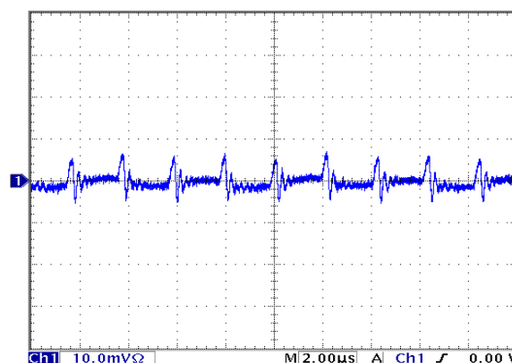
Figure 12: Input Terminal Ripple Current, i_c , at full rated output current and nominal input voltage with 4.7 \mu H source impedance and 100 \mu F electrolytic capacitor (100 mA/div). See Figure 11.
