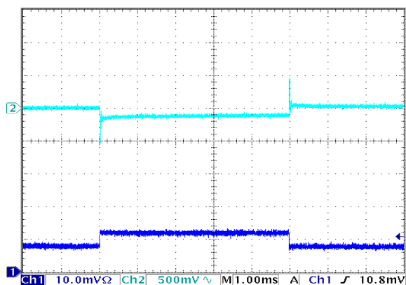
Figure 9: Output voltage response to step-change in load current (50%-75%-50% of I_{out(max)} ; dI/dt = 5A/\mu s ). Load cap: 1 \mu F ceramic and 10 \mu F tantalum capacitors. Top trace: Vout (500mV/div), Bottom trace: Iout (10A/div).
