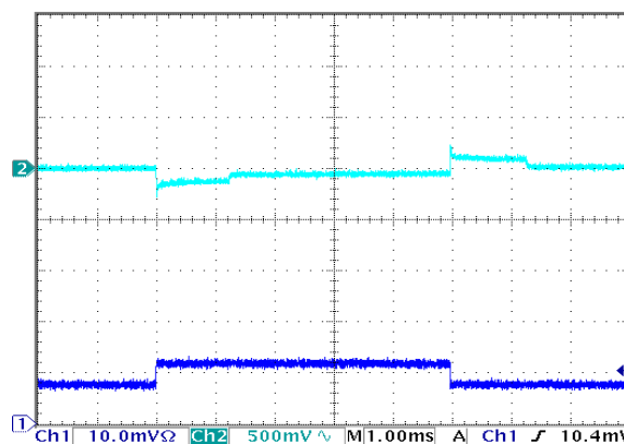
Figure 10: Output voltage response to step-change in load current (50%-75%-50% of I_{out(max)} ; dI/dt = 5A/\mu s ). Load cap: 470 \mu F , 15 mW ESR tantalum capacitor. Top trace: Vout (500mV/div), Bottom trace: Iout (10A/div).
