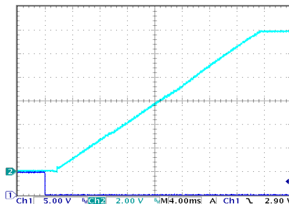
Figure 8: Turn-on transient at zero load (4ms/div). Ch 1: ON/OFF input (5V/div), Ch 2: Vout (2V/div)
