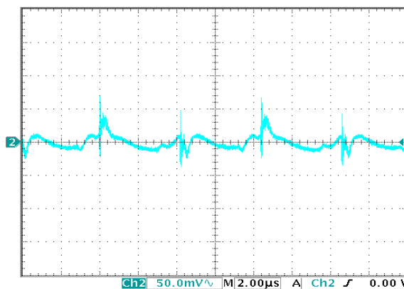
Figure 14: Output voltage ripple at nominal input voltage and rated load current (50mV/div). Load capacitance: 1µF ceramic capacitor and 10µF tantalum capacitor. Bandwidth: 500 MHz. See Figure 11.
