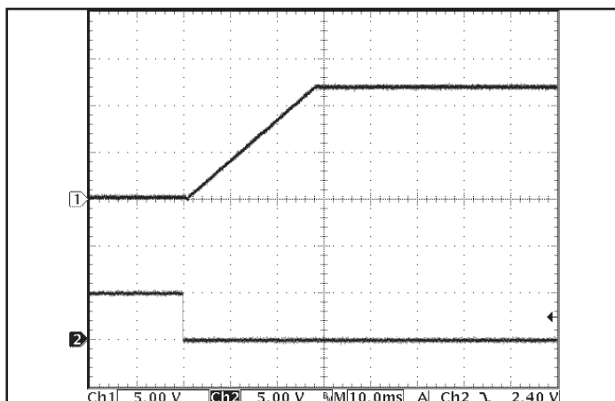
Figure 5: Turn-on Transient at zero load (10 ms/div). Ch 1: V out (5 V/div) Ch 2: ON/OFF input (5 V/div)
