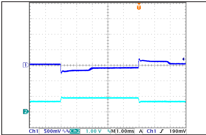
Figure 7: Output Voltage Response to Step-Change in Load Current (50%-75%-50% of I_{out(max)} ; dI/dt = 5 \text{ A}/\mu\text{s} ; 1 ms/div). Load cap: 470 \mu\text{F} electrolytic capacitor. Top trace: V_{out} (500 mV/div). Bottom trace: I_{out} (35 A/div).
