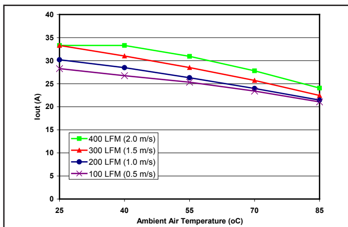
Figure 3: Thermal Derating (max output current vs. ambient air temperature) for airflow rates of 100LFM through 400LFM with air flowing from pin 3 to pin 1 (nominal input voltage - Base Plated Unit).
