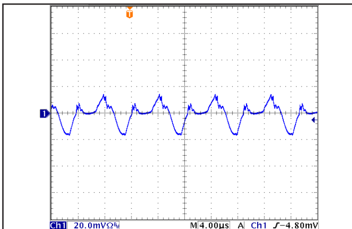
Figure 11: Output Ripple voltage at nominal input voltage and rated load current (20 mV/div; 4 \mu\text{s} /div). Load capacitance: 1 \mu\text{F} ceramic capacitor and 10 \mu\text{F} tantalum capacitor. Bandwidth: 20 MHz. See Figure 8.
