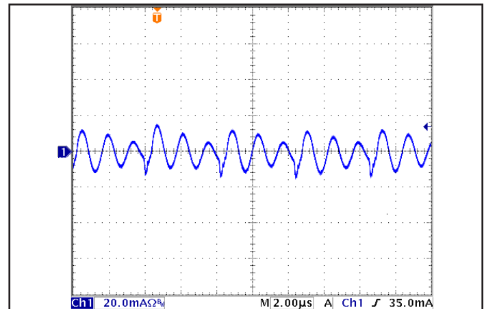
Figure 10: Input Reflected Ripple Current, i_s , through a 4.7 \mu\text{H} source inductor, using a 220 \mu\text{F} input capacitor, at nominal input voltage and rated load current (20 mA/div; 2 \mu\text{s} /div). See Figure 8.
