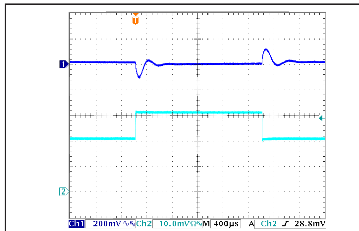
Figure 12: Output voltage response to step-change in load current (50%-75%-50% of I_{out(max)} ; dI/dt = 2A/\mu s ). Load cap: 330μF electrolytic output capacitance. Top trace: V_{out} (200mV/div). Bottom trace: I_{out} (1A/div).
