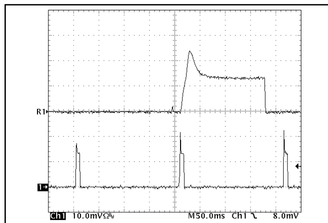
Figure 18: Load current (5A/div) as a function of time when the converter attempts to turn on into a 1\ m\ \Omega short circuit. Top trace (2.5ms/div) is an expansion of the on-time portion of the bottom trace.
