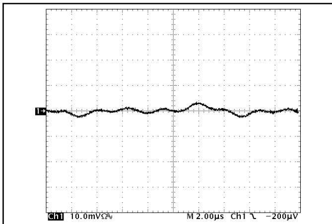
Figure 15: Input reflected ripple current, i_s , through a 10\ \mu H source inductor at nominal input voltage and rated load current (20 mA/div). See Figure 13.
