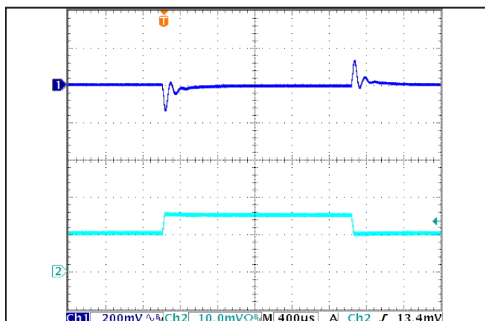
Figure 5: Output voltage response to step-change in load current (50%-75%-50% of Iout(max); dI/dt = 0.2 A/μs). Load cap: 1 μF ceramic and 15 μF tantalum capacitors. Ch 1: Vout, Ch 2: Iout (5A/div)
