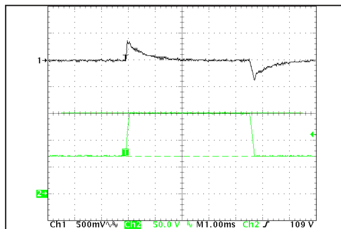
Figure 6: Output voltage response to step-change in input voltage (650V/ms), at Max. load current. Load cap: 15 \mu F tantalum cap and 1 \mu F ceramic cap. Ch 1: V_{out} , Ch 2: V_{in} .
