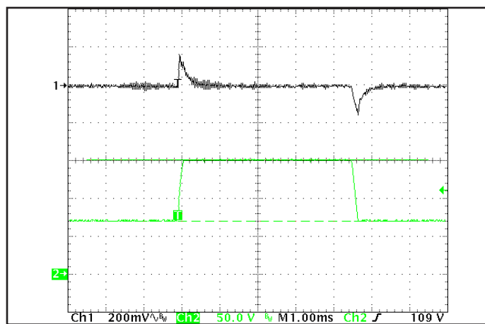
Figure 6: Output voltage response to step-change in input voltage (715V/ms), at Max. load current. Load cap: 15 \mu F tantalum cap and 1 \mu F ceramic cap. Ch 1: V_{out} , Ch 2: V_{in} .
