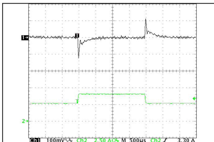
Figure 5: Output voltage response to step-change in load current (50%-75%-50% of I_{out(max)} ; dI/dt = 0.05A/\mu s . Load cap: 15 \mu F tantalum cap and 1 \mu F ceramic cap. Ch 1: V_{out} , Ch 2: I_{out} .
