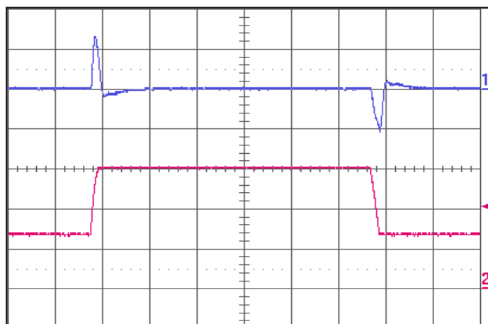
Figure 6: Output voltage response to step-change in input voltage (600 V/ms), at Max. load current. Load cap: 1\mu F ceramic cap. Ch 1: V_{out} (1V/div), Ch 2: V_{in} (50V/div), time scale: 1ms/div.
