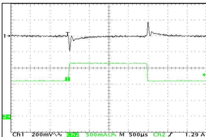
Figure 5: Output voltage response to step-change in load current (50%-75%-50% of I_{out(max)} ; dI/dt = 0.03A/\mu s . Load cap: 15 \mu F tantalum cap and 1 \mu F ceramic cap. Ch 1: V_{out} , Ch 2: I_{out} .
