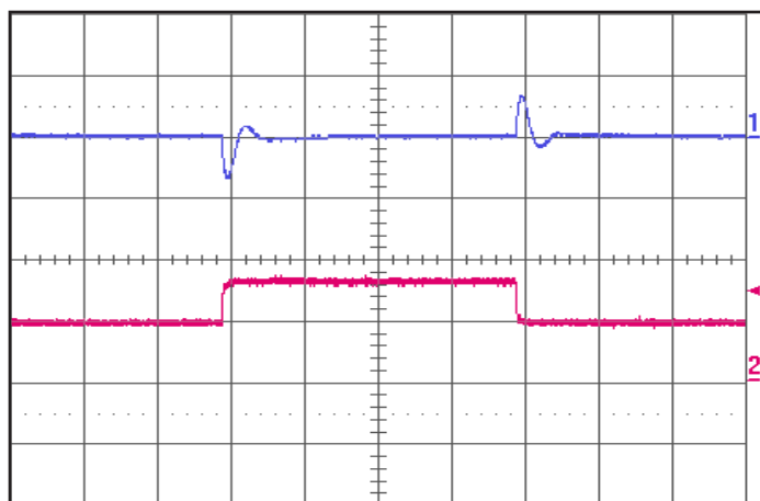
Figure 5: Output voltage response to step-change in load current (50%-75%-50% of I_{out(max)} ; dI/dt = 0.02A/\mu s . Load cap: 1\mu F ceramic cap. Ch 1: V_{out} (1V/div), Ch 2: I_{out} (500mA/div), time scale: 500 \mu s /div.
