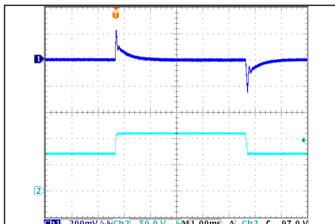
Figure 6: Output voltage response to step-change in input voltage (1000 V/ms, Vnom-Vmax-Vnom). Load cap: 1 μF ceramic and 15 μF tantalum capacitors. Ch 1: Vout, Ch 2: Vin.
