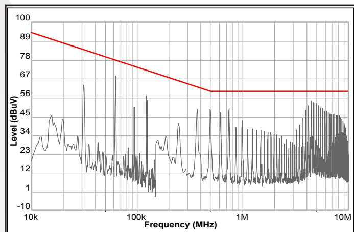
Figure 4: MIL-STD-461F Method CE102 High Frequency Conducted Emissions with two 33nF common mode capacitors. Limit line (in red) is the 'Basic Curve'. See MIL-STD-461 Compliance Matrix Table for test setup.
