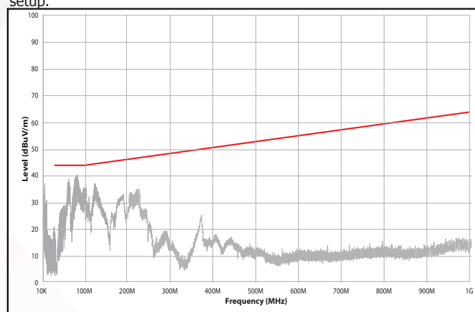
Figure 6: MIL-STD-461F Method RE102 High Frequency Radiated Emissions. Limit line (in red) is the 'Fixed Wing Internal, ≥ 25 meters Nose to Tail'. See MIL-STD-461 Compliance Matrix Table for test setup.
