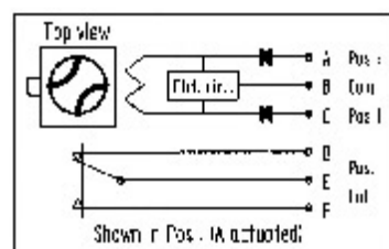
Latching Mechanism
