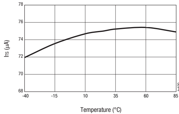
Figure 12. Current Source at the TS Pin vs Temperature (for Option AC, AD, AG, AH, AK, AL, BO, BP)
