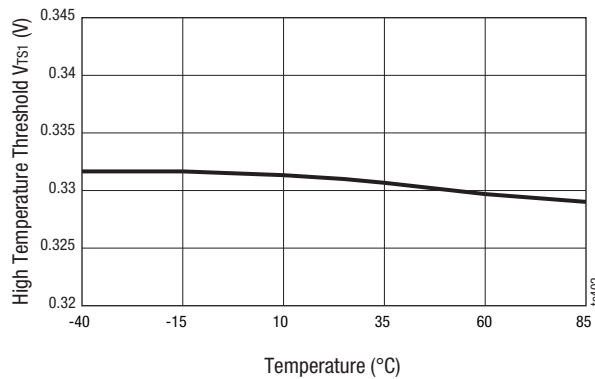
Figure 14. High Temperature Threshold vs Temperature (for Option AC, AD, AG, AH, AK, AL, BO, BP)
