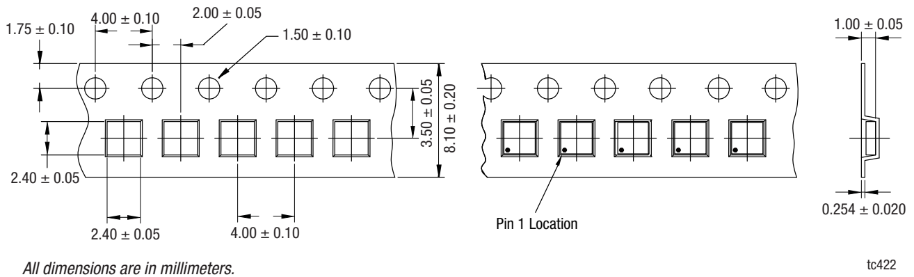
Figure 34. AAT3693 Tape and Reel Dimensions
