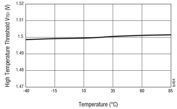
Figure 16. High Temperature Threshold vs Temperature (for Option AA, AB, AE, AF, AI, AJ, BM, BN; V_{IN} = 5\text{ V} )
