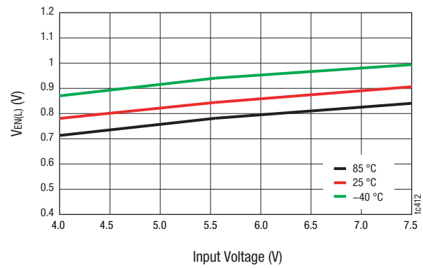
Figure 24. Input High Threshold vs Input Voltage
