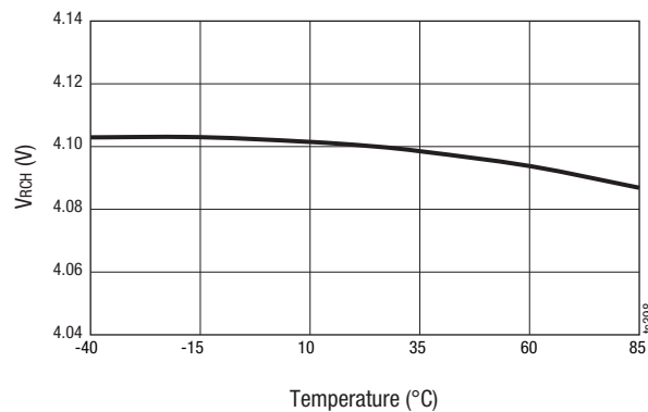
Figure 10. Battery Recharge Voltage Threshold vs Temperature
