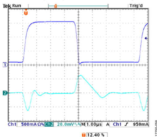
Figure 58. Output Transient Response, V_{\text{OUT}} = 5\text{ V} , C_{\text{OUT}} = 4.7\text{ }\mu\text{F}
