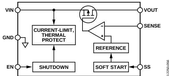
Figure 56. Internal Block Diagram
