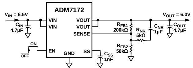
Figure 64. Noise Reduction Modification
