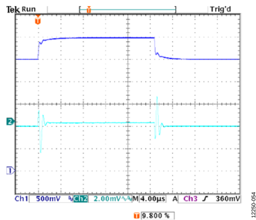
Figure 54. Line Transient Response, 2.5 V to 3 V, I_{LOAD} = 500 mA, Adjustable Version, V_{OUT} = 1.2 V, CH1 = V_{IN} , CH2 = V_{OUT}
