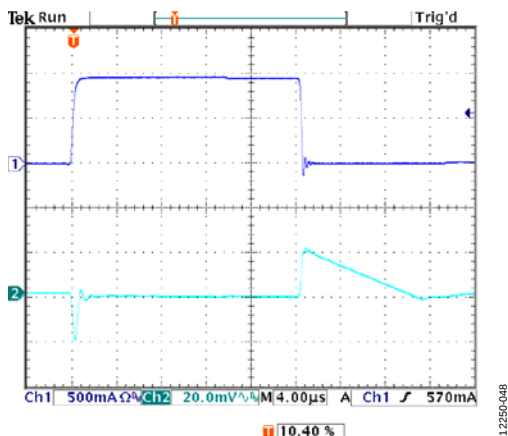
Figure 48. Load Transient Response, I_{LOAD} = 10\text{ mA} to 1\text{ A} , V_{OUT} = 5\text{ V} , V_{IN} = 5.5\text{ V} , CH1 = I_{LOAD} , CH2 = V_{OUT}
