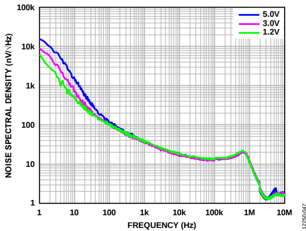
Figure 47. Output Noise Spectral Density, Different Output Voltages, Load Current = 100 mA
