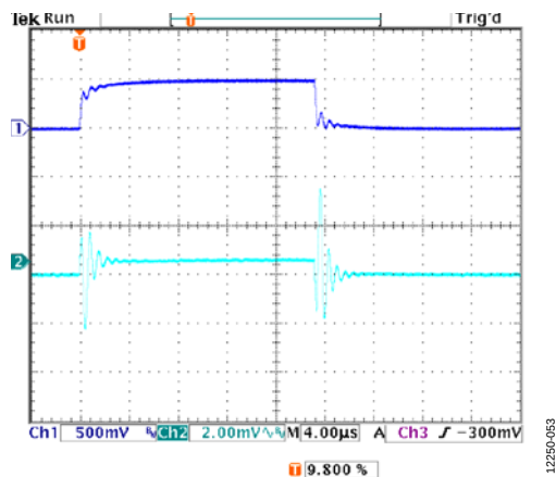
Figure 53. Line Transient Response, 6 V to 6.5 V, I_{LOAD} = 2 A, V_{OUT} = 5 V, CH1 = V_{IN} , CH2 = V_{OUT}
