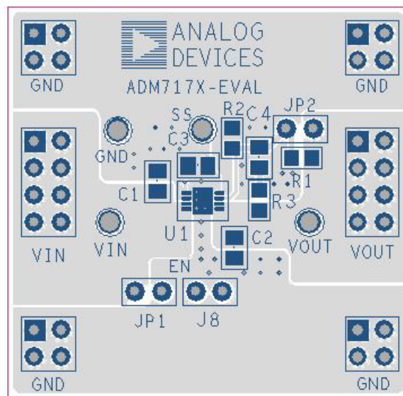
Figure 71. Example LFCSP PCB Layout
