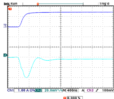
Figure 2. Transient Response (Trace 2), 1 mA to 1.5 A Load Step in 400 ns (Trace 1)
