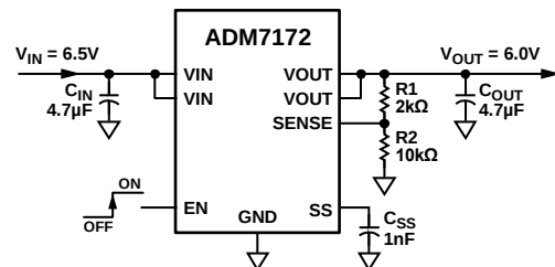
Figure 57. Typical Adjustable Output Voltage Application Schematic
