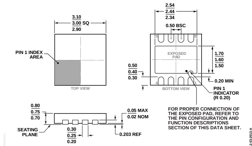
Figure 72. 8-Lead Lead Frame Chip Scale Package [LFCSP_WD] 3 mm × 3 mm Body, Very Very Thin, Dual Lead (CP-8-21) Dimensions shown in millimeters
