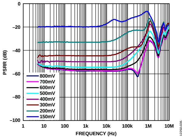
Figure 35. Power Supply Rejection Ratio (PSRR) vs. Frequency, V_{OUT} = 5\text{ V} , 2 A Load Current, Various Headroom Voltages
