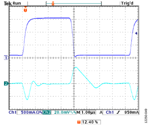
Figure 49. Load Transient Response, I_{LOAD} = 100\text{ mA} to 1.6\text{ A} , V_{OUT} = 5\text{ V} , V_{IN} = 5.5\text{ V} , CH1 = I_{LOAD} , CH2 = V_{OUT}
