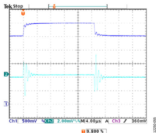
Figure 55. Line Transient Response, 2.5 V to 3 V, I_{LOAD} = 2 A, Adjustable Version, V_{OUT} = 1.2 V, CH1 = V_{IN} , CH2 = V_{OUT}
