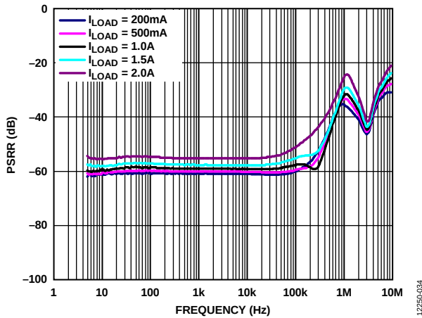
Figure 34. Power Supply Rejection Ratio (PSRR) vs. Frequency, 300 mV Headroom, V_{OUT} = 3\text{ V}
