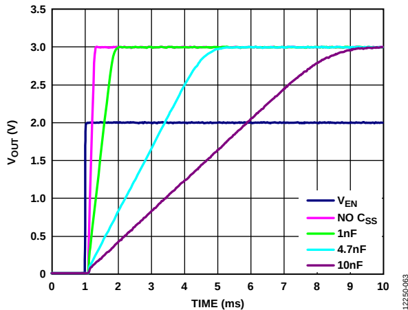
Figure 63. Typical Soft Start Behavior, Different C_{SS} Values
