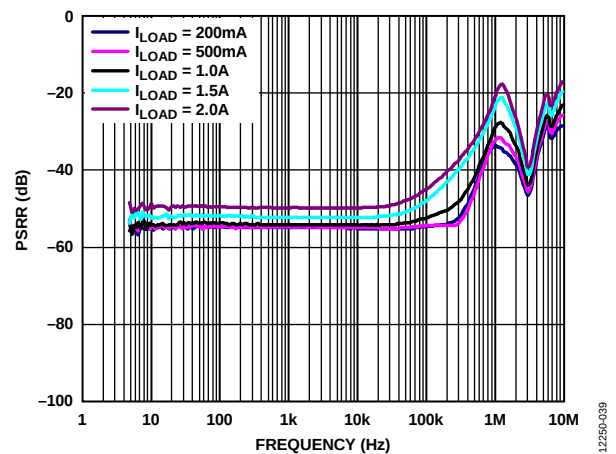
Figure 39. Power Supply Rejection Ratio (PSRR) vs. Frequency, 300 mV Headroom, V_{OUT} = 5\text{ V}
