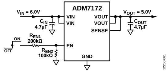
Figure 61. Typical EN Pin Voltage Divider
