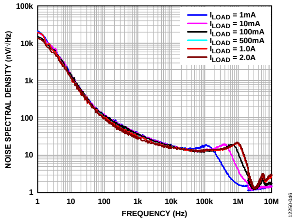
Figure 46. Output Noise Spectral Density, V_{OUT} = 5\text{ V}
