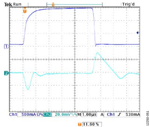
Figure 51. Load Transient Response, I_{LOAD} = 100\text{ mA} to 1.6\text{ A} , Adjustable Version, V_{OUT} = 1.2\text{ V} , V_{IN} = 2.5\text{ V} , CH1 = I_{LOAD} , CH2 = V_{OUT}
