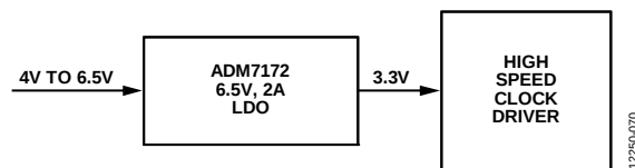
Figure 69. Clock Driver Power
