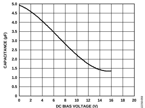
Figure 59. Capacitance vs. DC Bias Voltage
