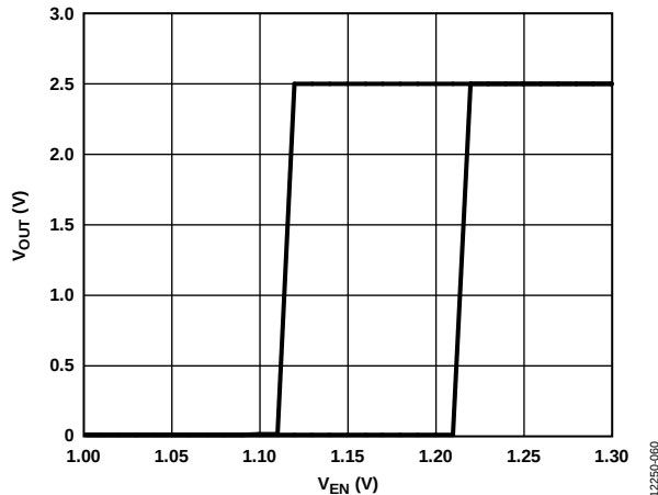
Figure 60. Typical V_{OUT} Response to EN Pin Operation
