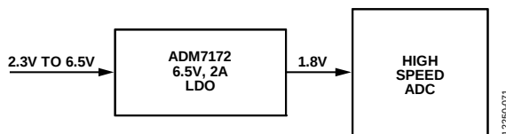
Figure 70. High Speed ADC Power
