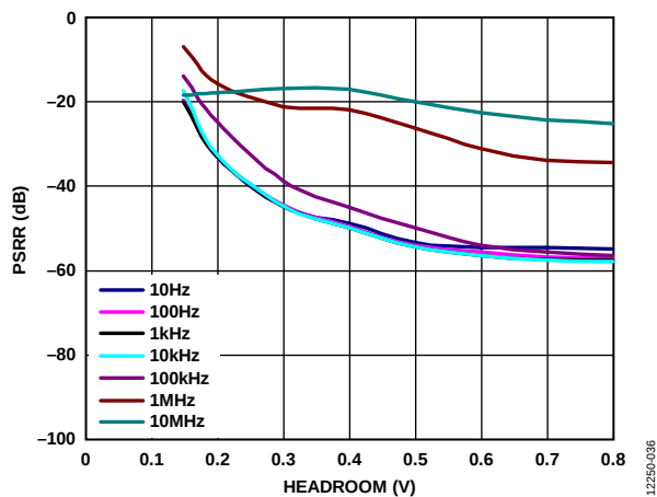
Figure 36. Power Supply Rejection Ratio (PSRR) vs. Headroom, V_{OUT} = 5\text{ V} , 2 A Load Current, Different Frequencies
