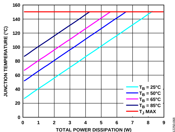
Figure 68. LFCSP Power Dissipation for Various Board Temperatures
