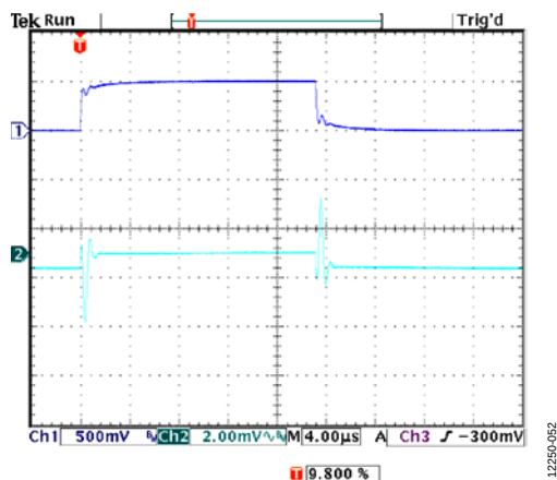
Figure 52. Line Transient Response, 6 V to 6.5 V, I_{LOAD} = 500 mA, V_{OUT} = 5 V, CH1 = V_{IN} , CH2 = V_{OUT}
