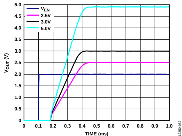
Figure 62. Typical Start-Up Behavior
