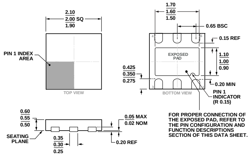
Figure 67. 6-Lead Lead Frame Chip Scale Package [LFCSP_UD] 2.00 mm × 2.00 mm Body, Ultra Thin, Dual Lead (CP-6-3) Dimensions shown in millimeters
