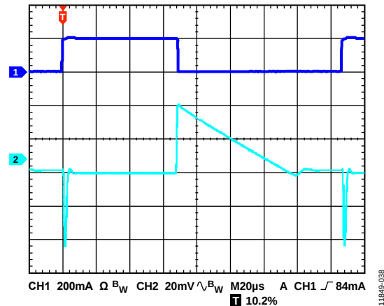
Figure 40. Load Transient Response, I_{LOAD} = 1\text{ mA} to 200\text{ mA} , V_{OUT} = 1.8\text{ V} , V_{IN} = 3\text{ V} , CH1 Load Current, CH2 V_{OUT}
