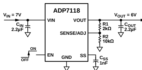
Figure 43. Typical Adjustable Output Voltage Application Schematic
