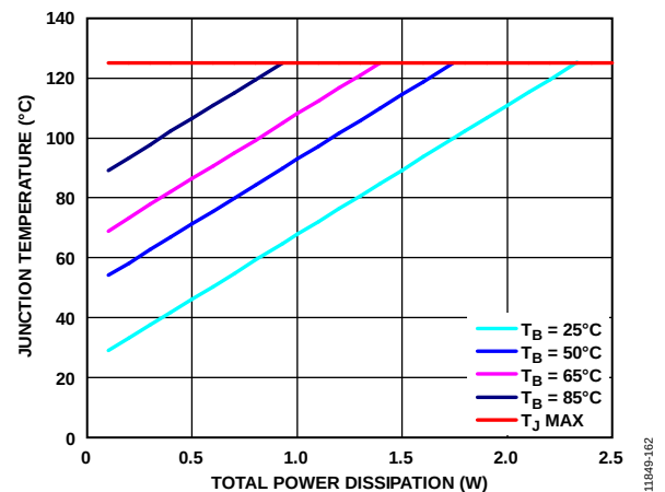
Figure 63. TSOT Junction Temperature Rise, Different Board Temperatures
