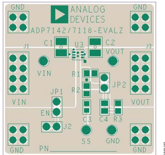
Figure 64. Example LFCSP PCB Layout
