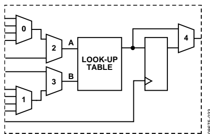
Figure 39. PLA Element
