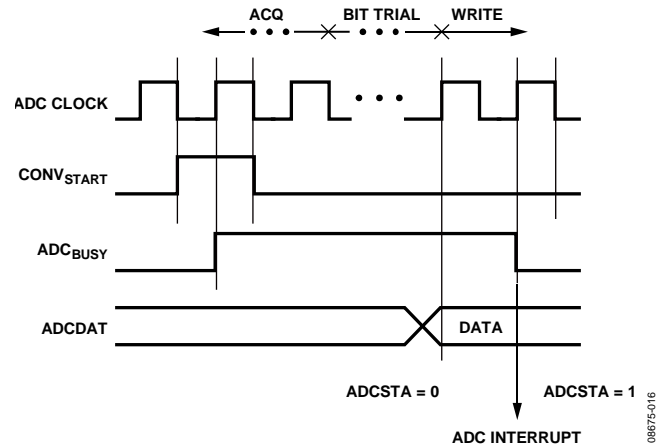
Figure 23. ADC Timing
