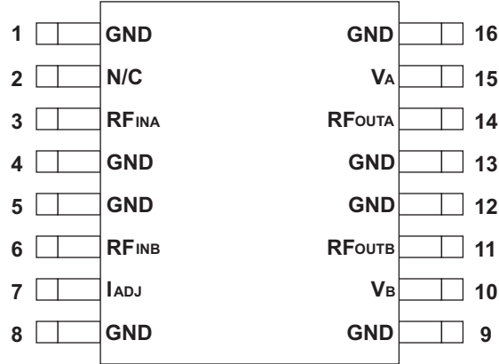
Figure 2: Pin Out
