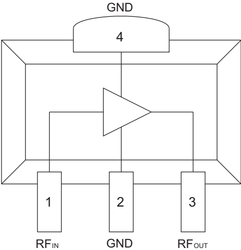
Figure 2: Pinout
