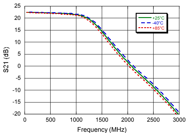
Gain to 3000 MHz
