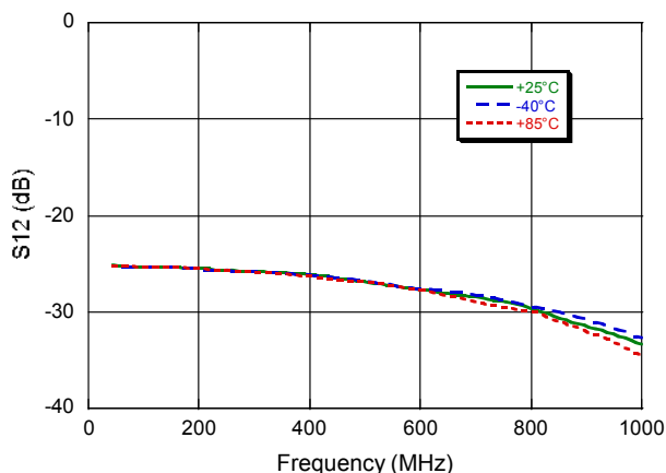
Reverse Isolation
