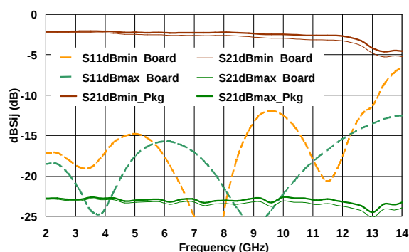
PCB Measured performances @ 20°C
