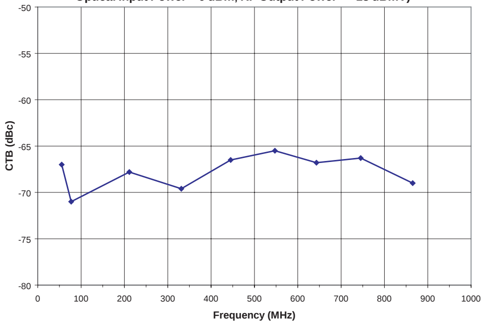
Figure 12: CTB vs. Frequency ( T_A = +25^\circ\text{C} , V_{CC} = +5\text{ V} , 132 Analog Channel Loading, Optical Input Power = 0 dBm, RF Output Power = +18 dBmV)
