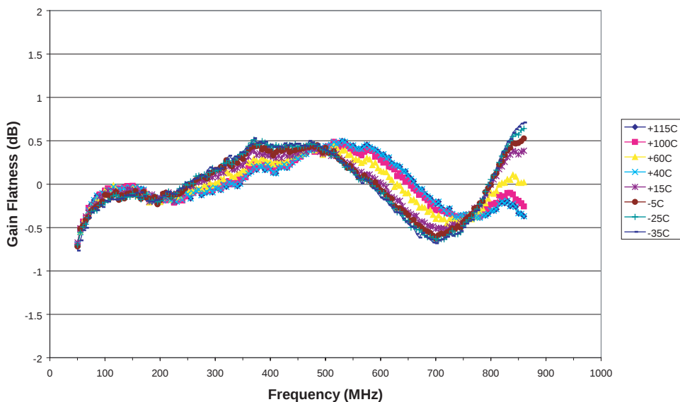
Figure 10: Gain Flatness To Best Fit Line vs. Frequency over Temperature ( V_{CC} = +5\text{ V} , V_{AGC} = 0\text{ V} )
