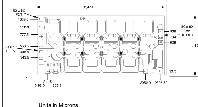
Chip Diagram
