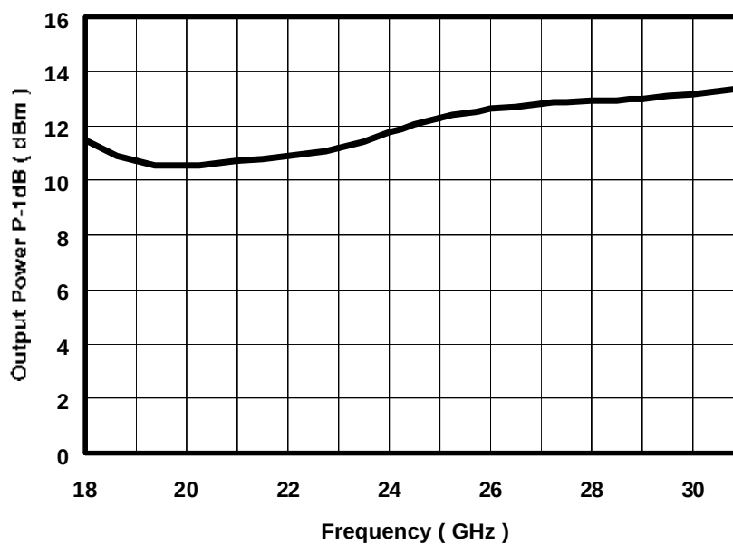
Typical Poutput Power -1dB measurements on wafer.
