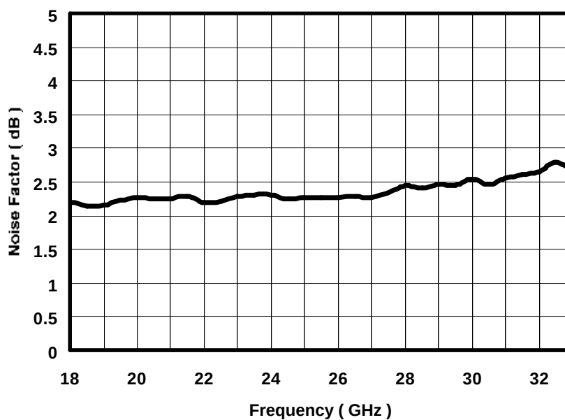
Typical NOISE Figure measurements in test-jig.
