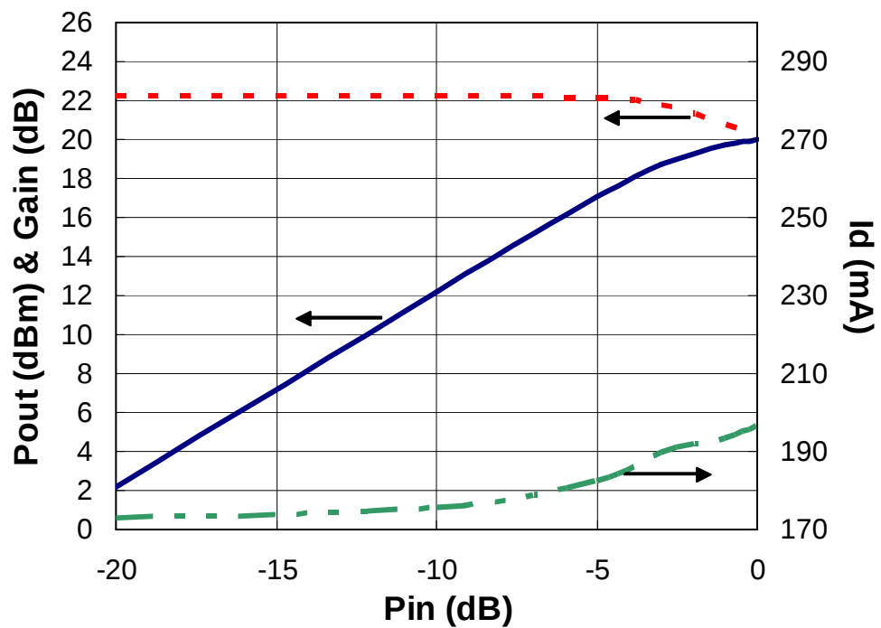
Pout, Gain &amp; Id versus Pin @ 7GHz
