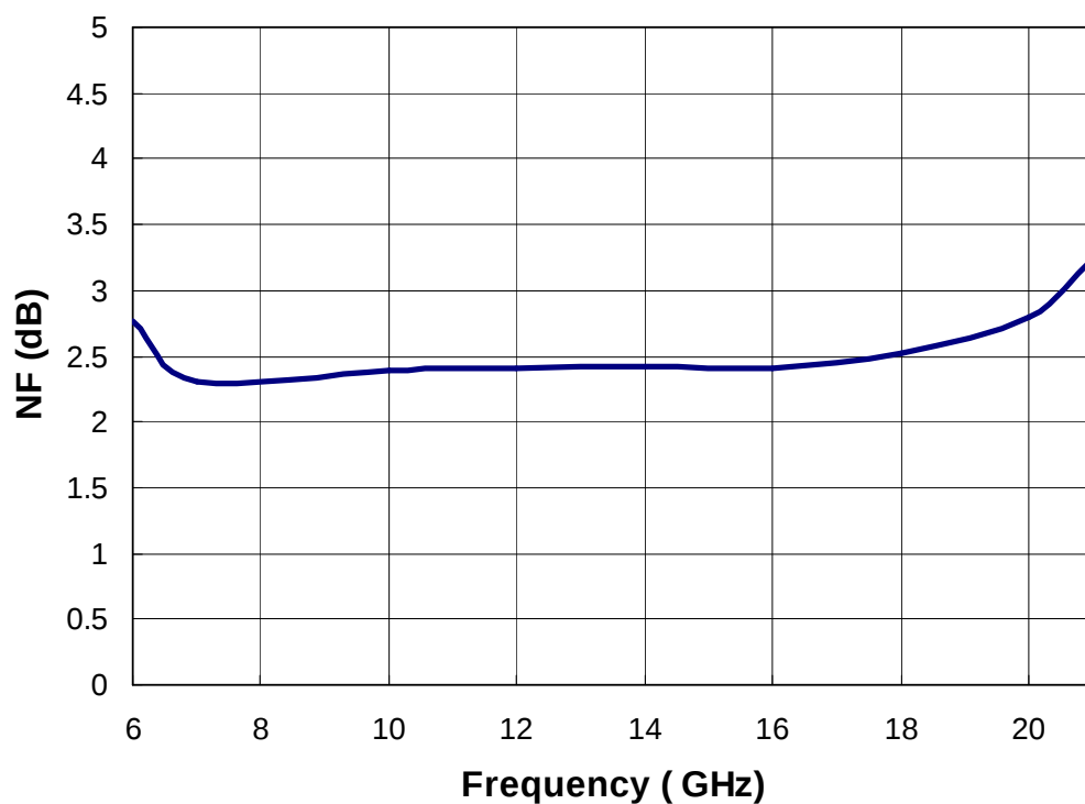
Noise figure versus frequency
