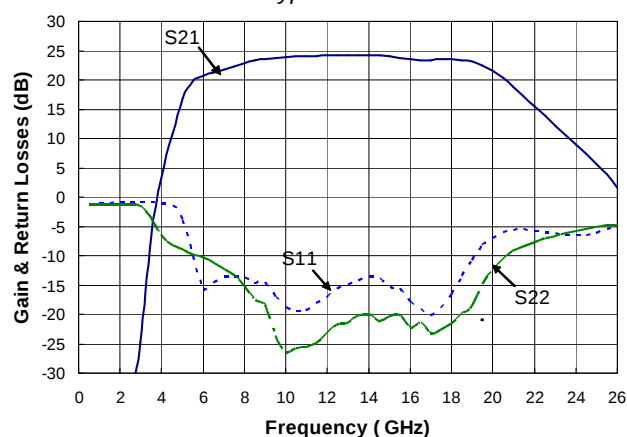
On wafer typical measurements
