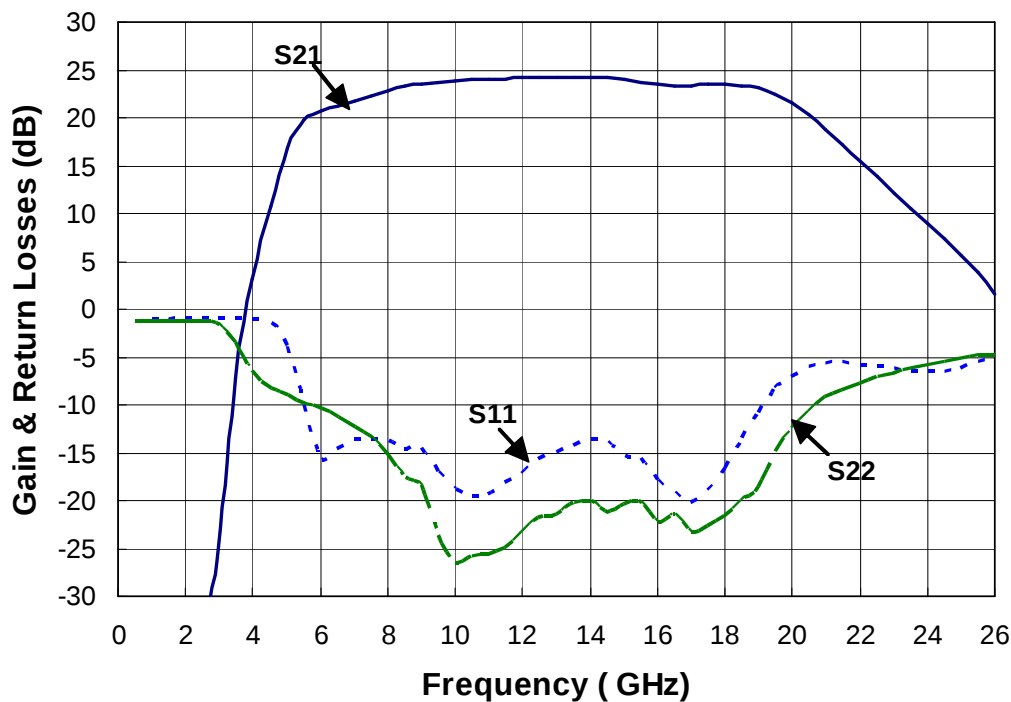
Gain & return losses versus frequency
