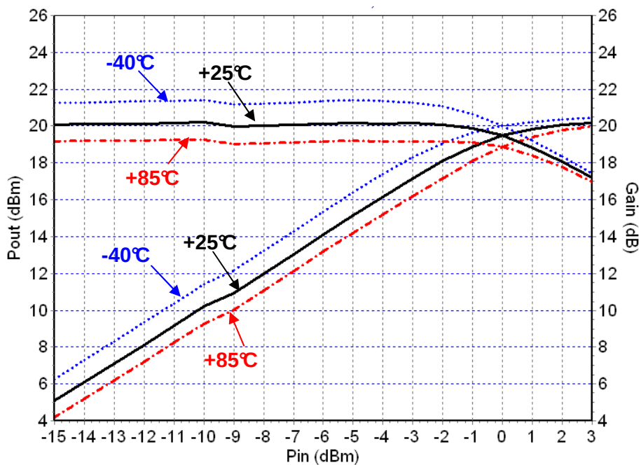
Gain and Pout versus frequency and temperature @ 7GHz
