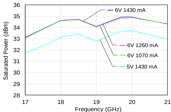
Saturated Power vs. Frequency vs. Bias
