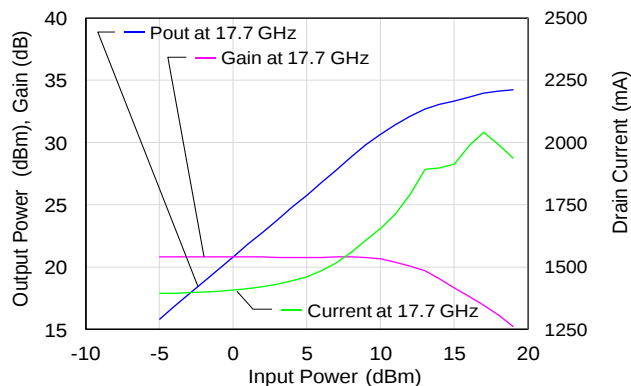
17.7 GHz Power, Gain, and Current vs. Input Power
