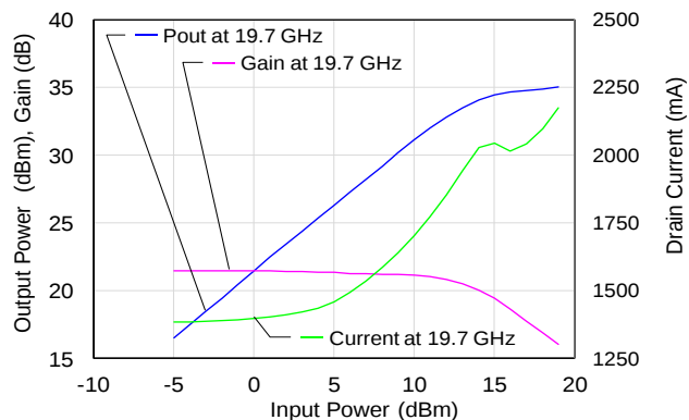
19.7 GHz Power, Gain, and Current vs. Input Power
