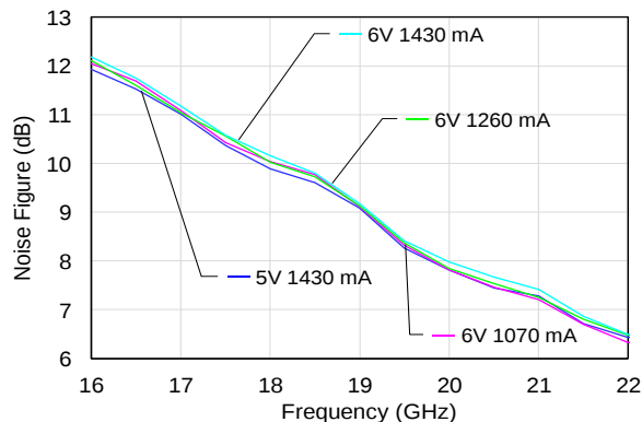
Noise Figure vs. Frequency vs. Bias
