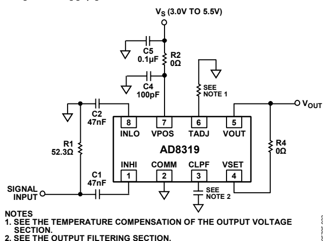
Figure 22. Basic Connections
