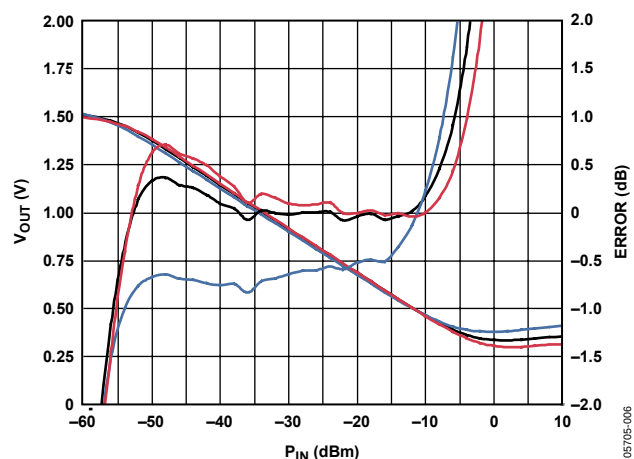
Figure 6. V_{OUT} and Log Conformance Error vs. Input Amplitude at 3.6 GHz, R_{TADJ} = 8\text{ k}\Omega
