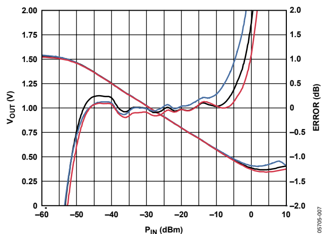
Figure 7. V_{OUT} and Log Conformance Error vs. Input Amplitude at 5.8 GHz, R_{TADJ} = 500\text{ }\Omega
