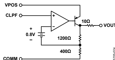
Figure 24. Output Interface
