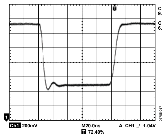
Figure 17. V_{OUT} Pulse Response Time; Pulsed RF Input 0.1 GHz, -10 dBm; C_{LPF} = \text{Open} ; R_{LOAD} = 150 \Omega
