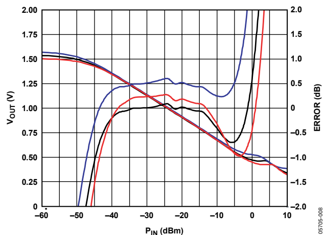
Figure 8. V_{OUT} and Log Conformance Error vs. Input Amplitude at 8.0 GHz, R_{TADJ} = \text{Open} , Error Calculated from P_{IN} = -34\text{ dBm} to P_{IN} = -16\text{ dBm}
