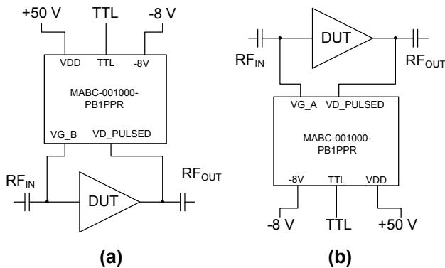
Figure 2. Pulsed Gate/Pulsed Drain Biasing: (b) North Biasing; (b) South Biasing
