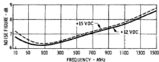
Noise Figure
