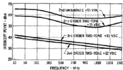
Intercept Point
