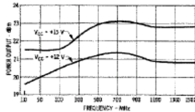
Power Output*
