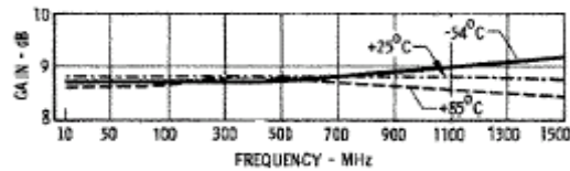
Gain
