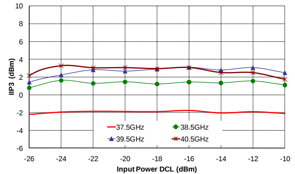
Input IP3 vs RF frequency at IF 3.5GHz
