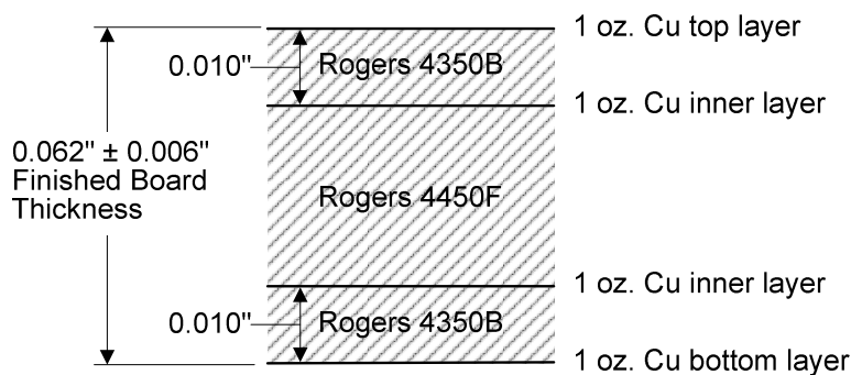
TriQuint PCB 1084112 Material and Stack-up
