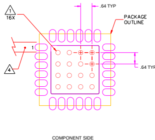
COMPONENT SIDE
