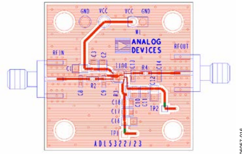
Figure 17. Evaluation Board Component Side View
