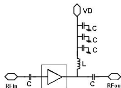
Figure 1. Simplified Schematic diagram
