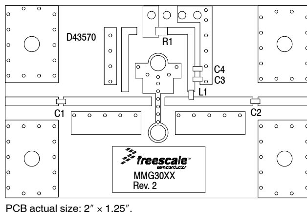
Figure 3. 50 Ohm Test Circuit Component Layout
