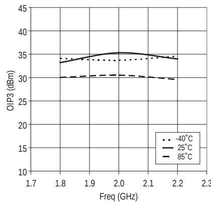
Figure 16. OIP3 vs Frequency and temperature
