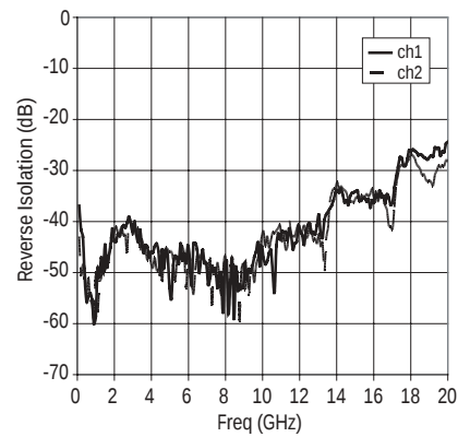
Figure 13. Isolation vs Frequency and channel
