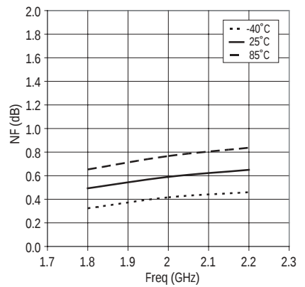
Figure 14. NF vs Frequency and temperature
