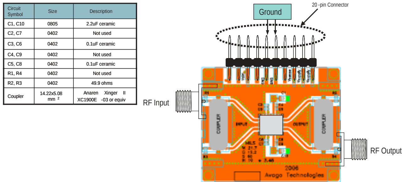
Figure 7. Suggested Balanced Amplifier Demo Board Layout Recommended PCB material is 10 mils Rogers RO4350. Suggested component values may vary according to layout and PCB material.
