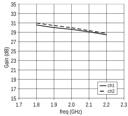
Figure 10. Gain vs Frequency and channel
