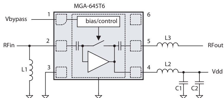
Figure 18. Demo Board Schematic Diagram
