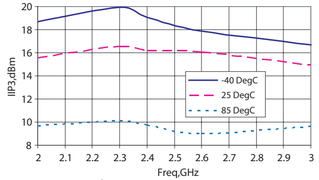
Figure 16. Bypass Mode IIP3 vs Frequency vs Temperature
