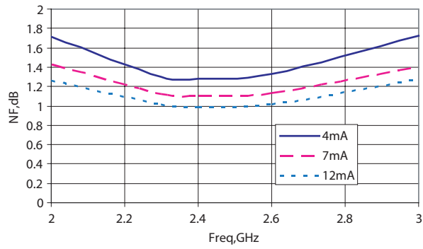
Figure 20. LNA Mode Noise Figure vs Frequency vs Id
