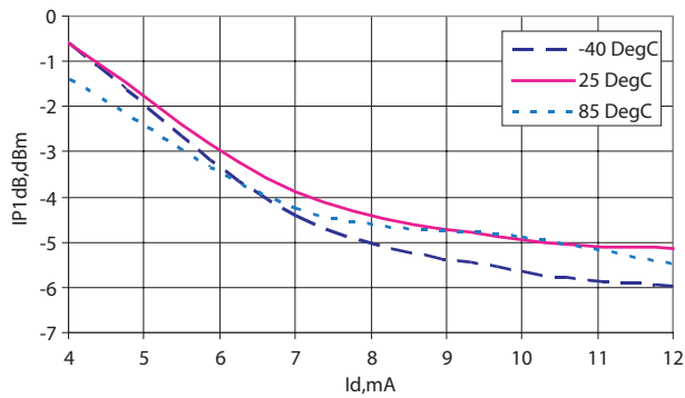
Figure 24. LNA Mode IP1dB vs Id vs Temperature
