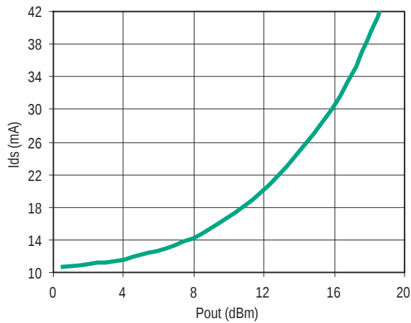
Figure 53. Ids vs Pout (Vd = 3V)
