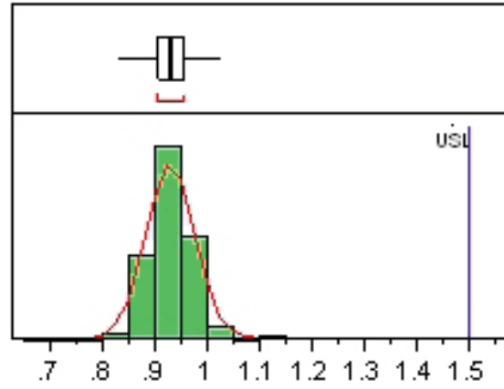
Figure 3. NF @ 0.5GHz 3V, Nominal=0.93, USL=1.50
