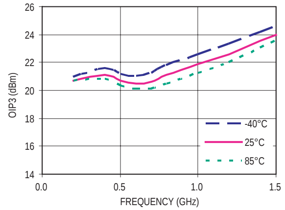
Figure 22. OIP3 vs Frequency ( V_d = 3V , I_{ds} = 15mA )
