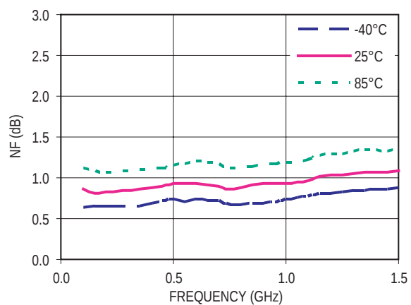
Figure 16. NF vs Frequency ( V_d = 3V , I_{ds} = 10mA )
