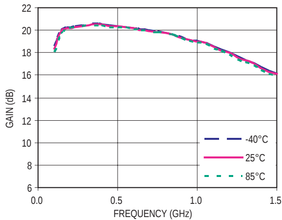
Figure 41. Gain vs Frequency ( V_d = 5V , I_{ds} = 15mA )
