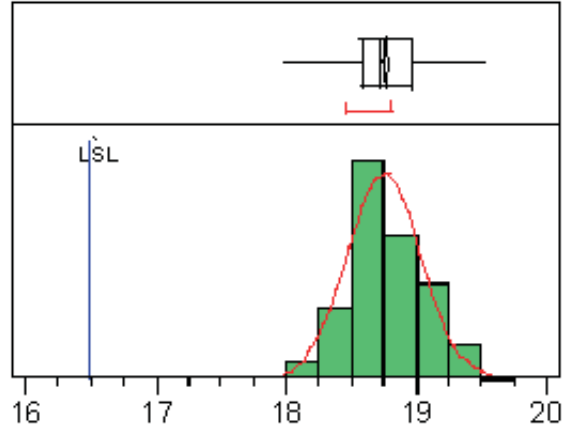
Figure 5. OIP3 @ 0.5GHz 3V, LSL=16.5, Nominal=18.7
