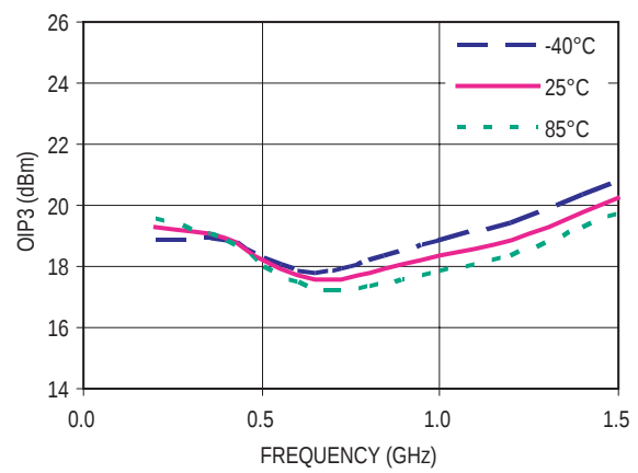
Figure 34. OIP3 vs Frequency ( V_d = 5V , I_{ds} = 10mA )
