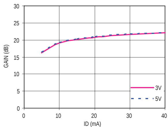
Figure 47. Gain vs Id( 500 MHz )
