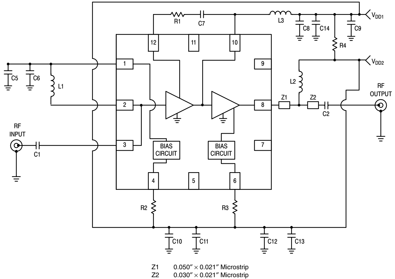
Figure 21. MML09212HT1 Test Circuit Schematic
