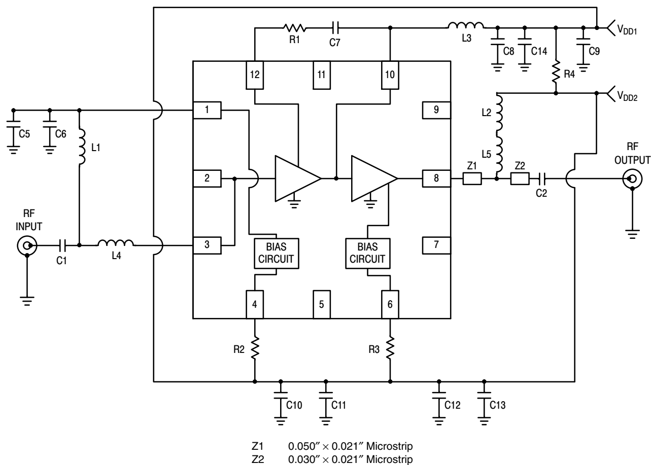
Figure 13. MML09212HT1 Test Circuit Schematic
