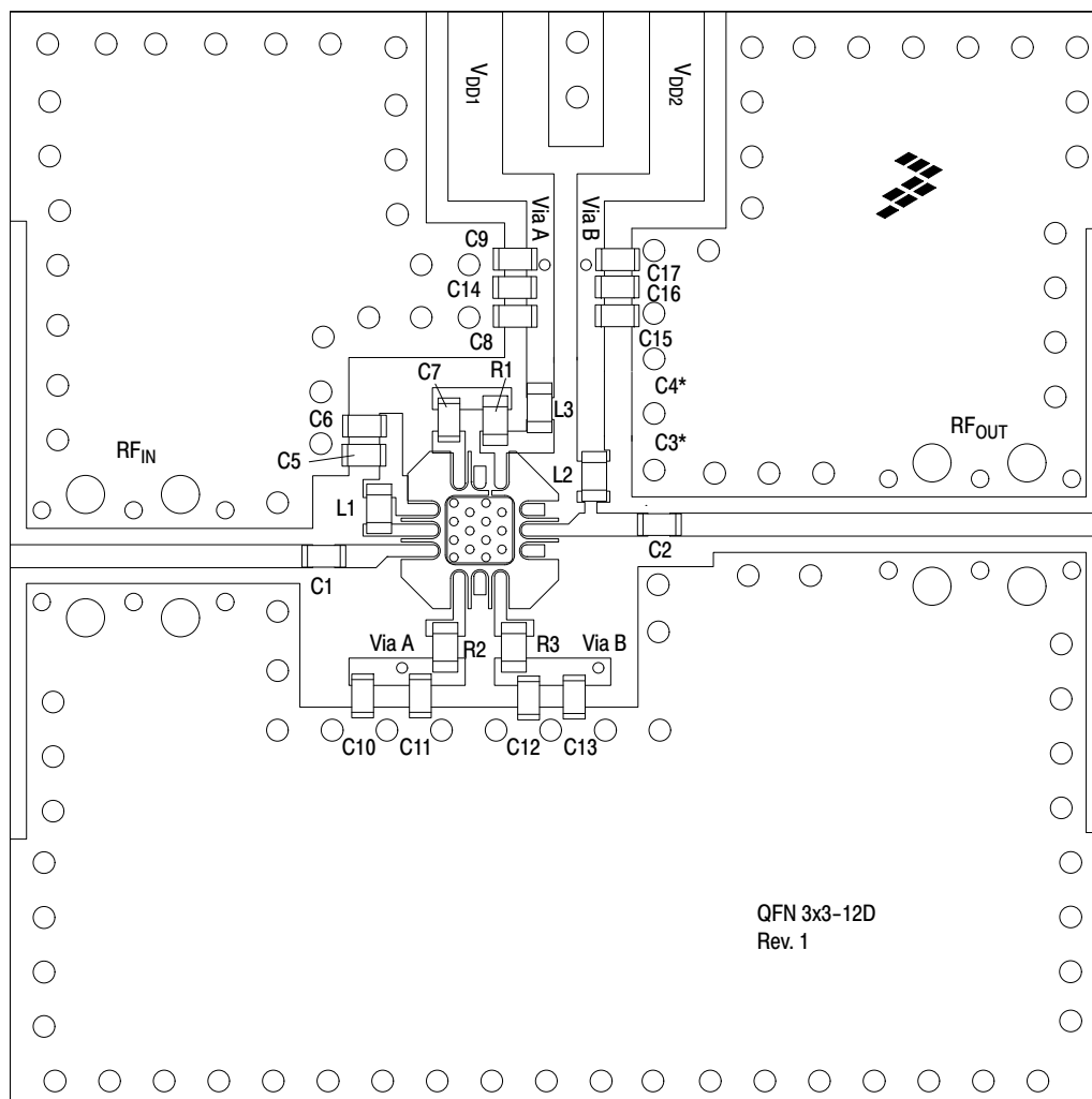
Figure 32. MML09212HT1 Test Circuit Component Layout
