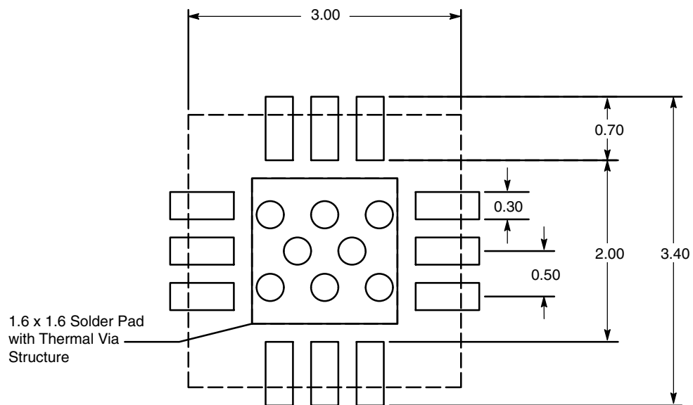
Figure 29. PCB Pad Layout for QFN 3 × 3
