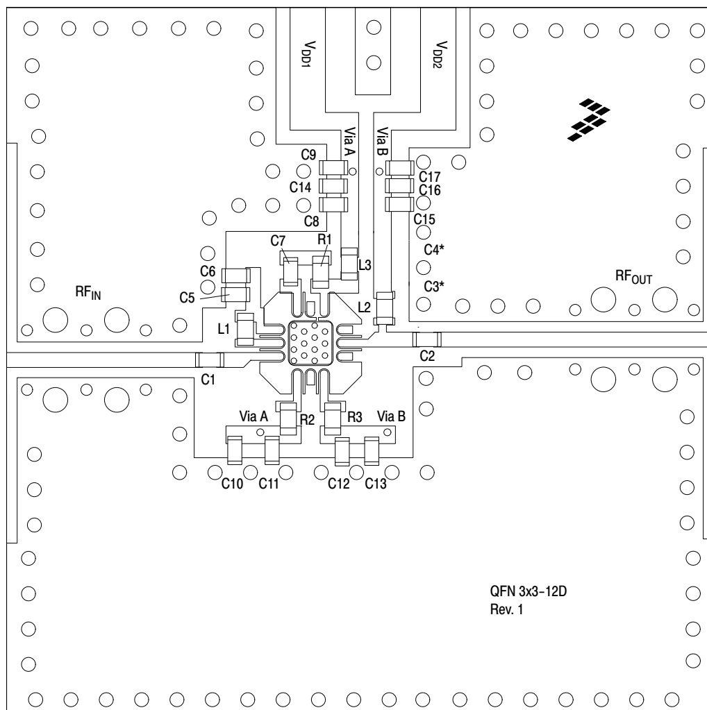
Figure 36. MML09212HT1 Test Circuit Component Layout
