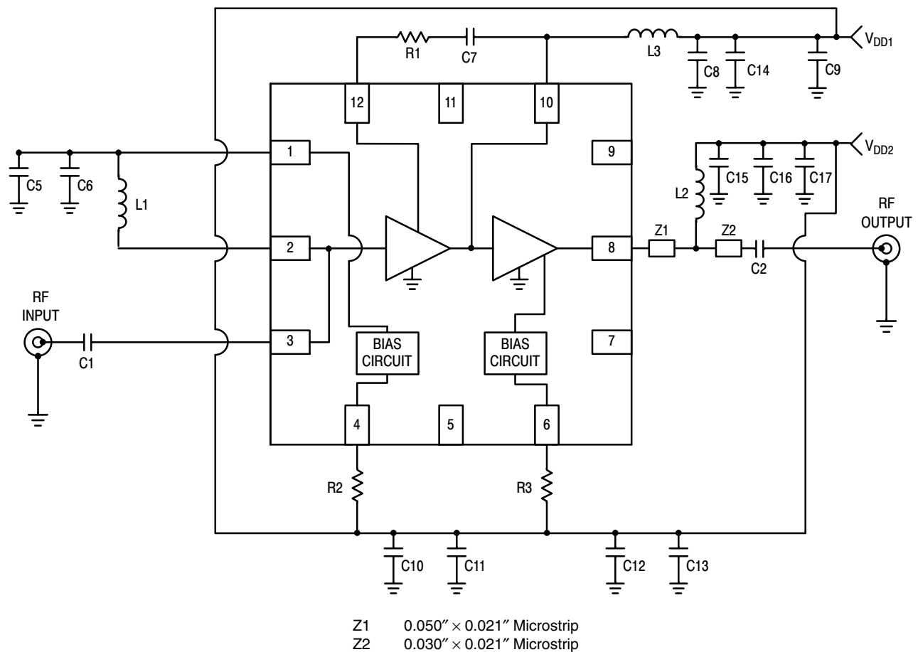
Figure 33. MML09212HT1 Test Circuit Schematic
