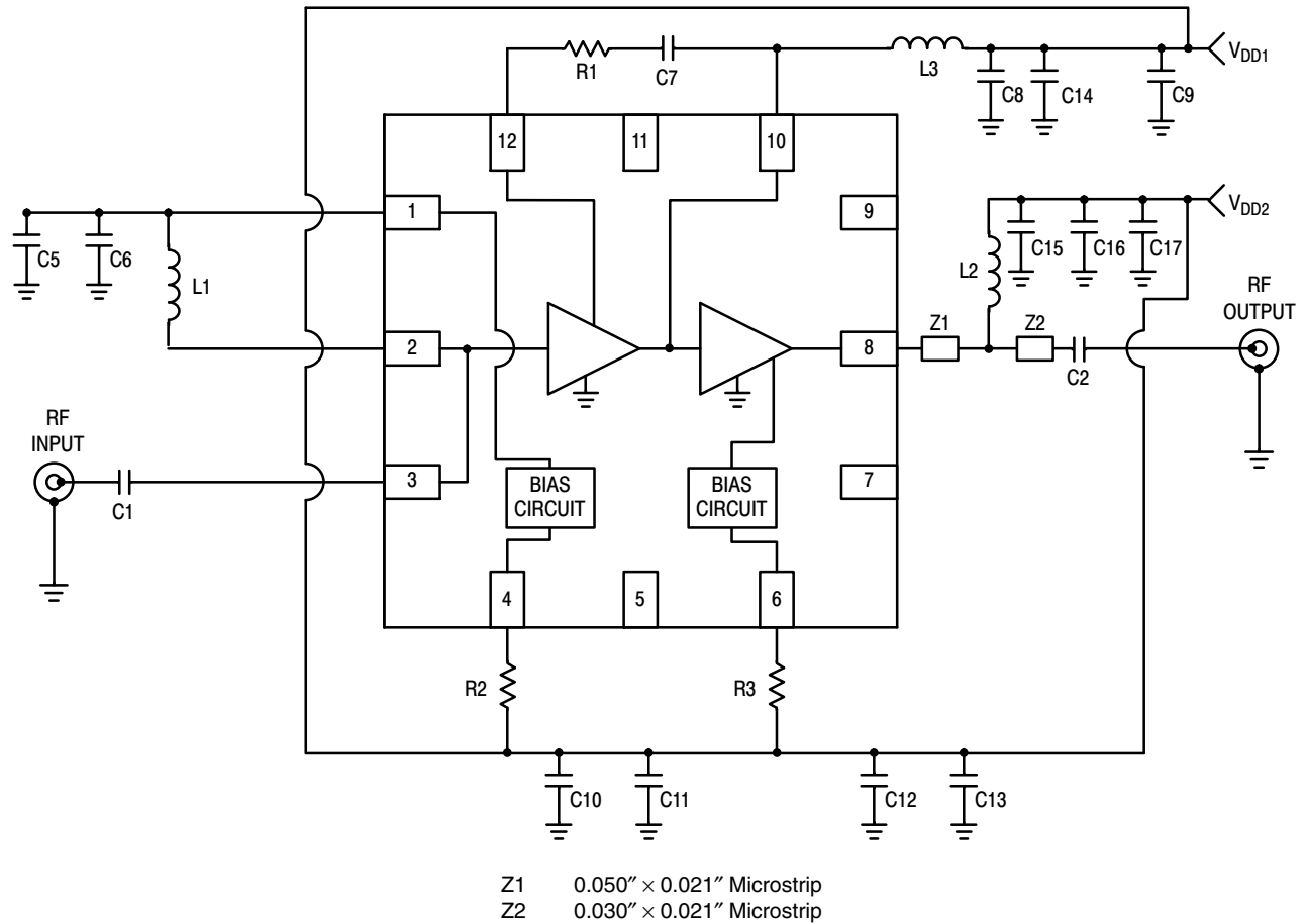
Figure 31. MML09212HT1 Test Circuit Schematic
