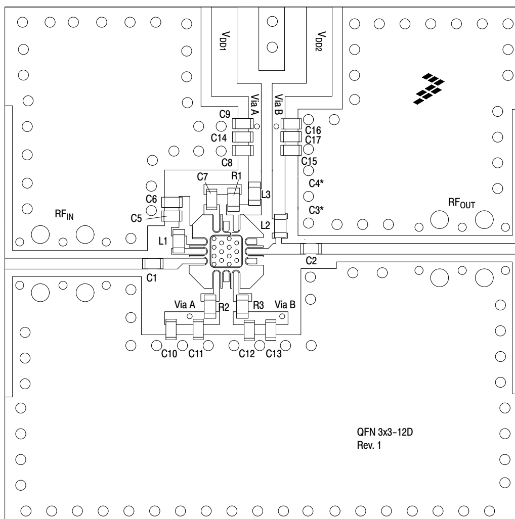
Figure 34. MML09212HT1 Test Circuit Component Layout
