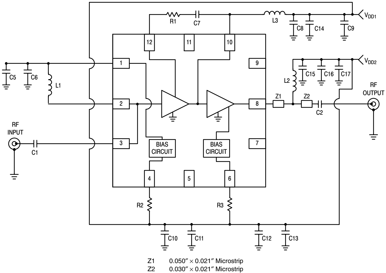
Figure 35. MML09212HT1 Test Circuit Schematic
