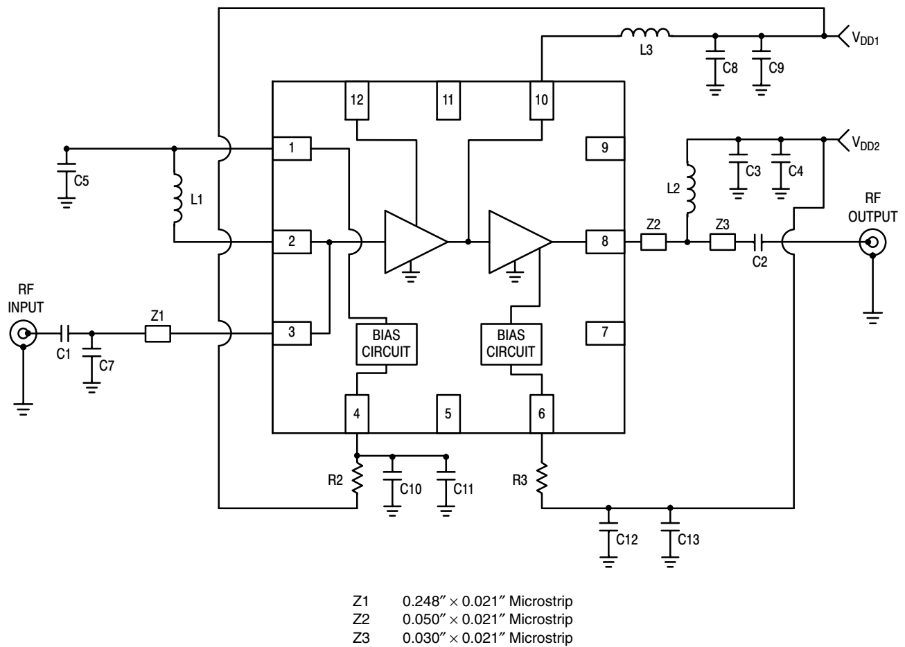
Figure A-3. MML20242HT1 Test Circuit Schematic
