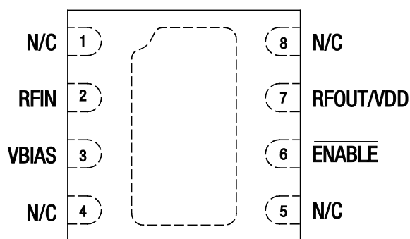
Figure 2. SKY67022-396LF Pinout – 8-Pin DFN (Top View)
