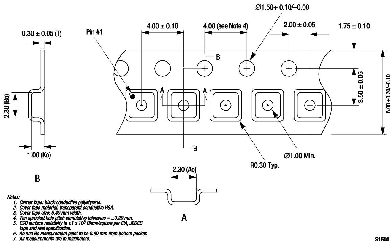
Figure 27. SKY67022-396LF Tape and Reel Dimensions
